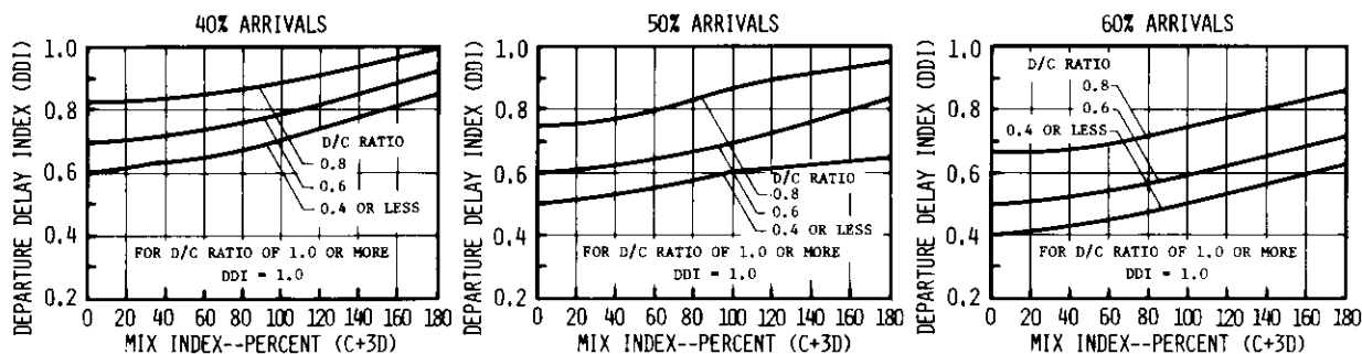
FIGURE 2-80 DELAY INDICES FOR RUNWAY USE DIAGRAM NO. 29 FOR VFR CONDITIONS
