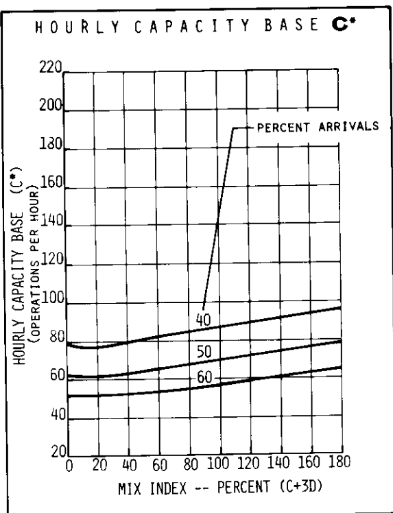
FIGURE 2-55 HOURLY CAPACITY OF RUNWAY USE DIAGRAMS NOS. 19, 30 FOR IFR CONDITIONS
