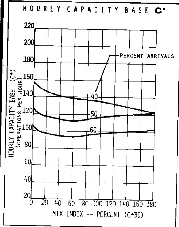
FIGURE 2-53 HOURLY CAPACITY OF RUNWAY USE DIAGRAMS NOS. 17, 20, 25, 31, 36 FOR IFR CONDITIONS
