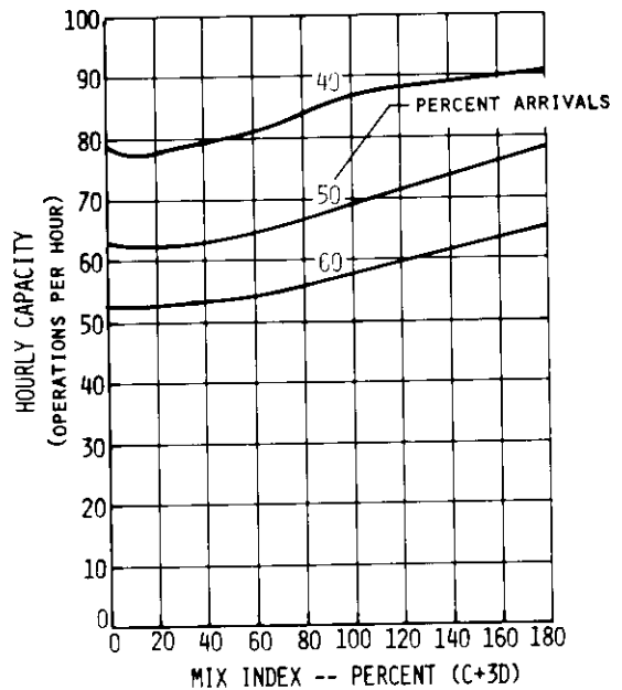
FIGURE A2-11 HOURLY CAPACITY OF RUNWAY USE DIAGRAM NO. 11
