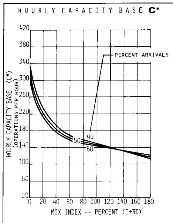
FIGURE 2-17 HOURLY CAPACITY OF RUNWAY USE DIAGRAMS NOS. 27, 28, 91, 116 FOR VFR CONDITIONS
