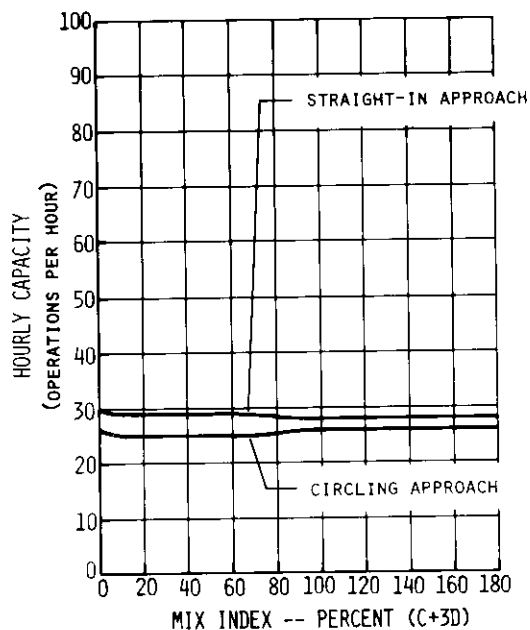
FIGURE A3-2B HOURLY CAPACITY IN NONRADAR ENVIRONMENT
