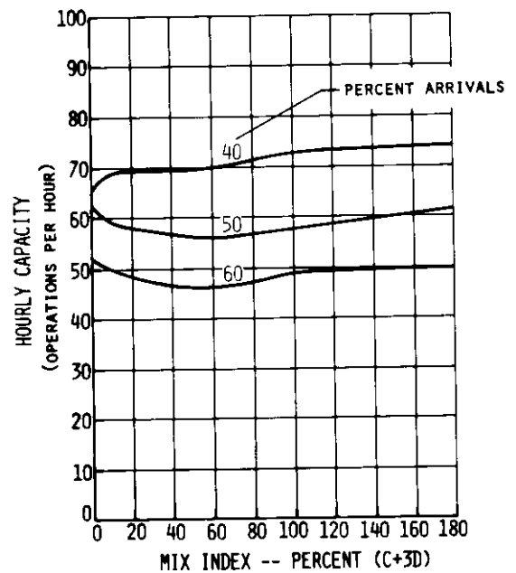
FIGURE A2-5 HOURLY CAPACITY OF RUNWAY USE DIAGRAM NO. 4
