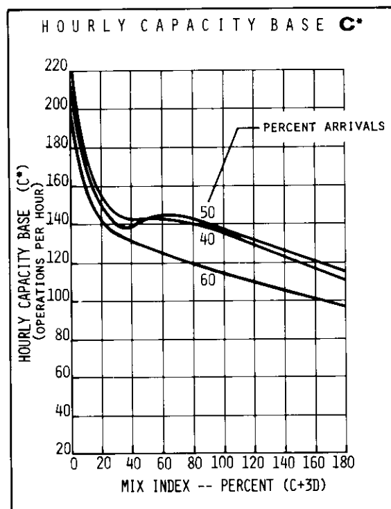
FIGURE 2-36 HOURLY CAPACITY OF RUNWAY USE DIAGRAMS NOS. 58, 64 FOR VFR CONDITIONS
