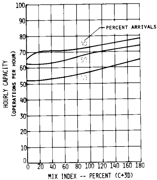
FIGURE A2-10 HOURLY CAPACITY OF RUNWAY USE DIAGRAM NO. 10
