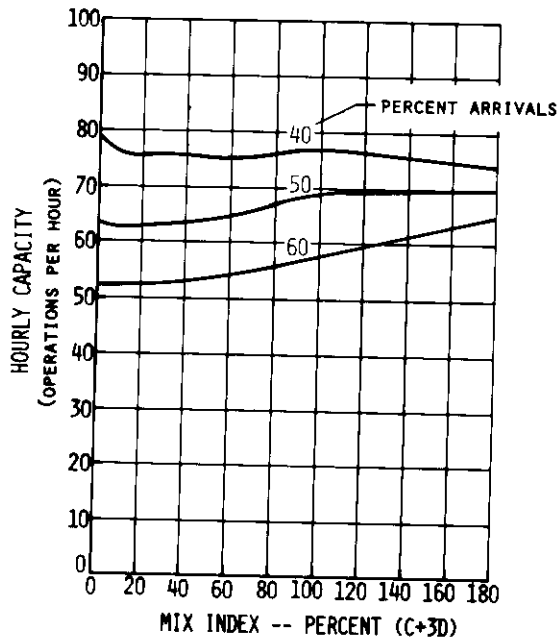
FIGURE A2-8 HOURLY CAPACITY OF RUNWAY USE DIAGRAM NO. 7b
