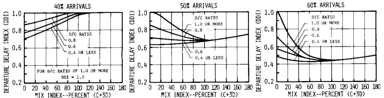
FIGURE 2-84 DELAY INDICES FOR RUNWAY USE DIAGRAMS NOS. 43, 49, 55, 61 FOR VFR CONDITIONS
