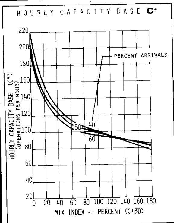
FIGURE 2-8 HOURLY CAPACITY OF RUNWAY USE DIAGRAMS NOS. 7, 8, 79, 104 FOR VFR CONDITIONS
