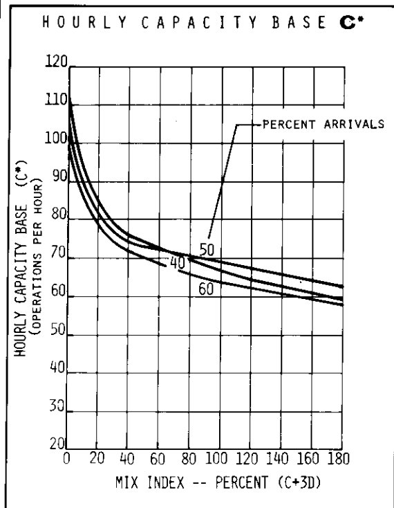
FIGURE 2-29 HOURLY CAPACITY OF RUNWAY USE DIAGRAMS NOS. 45, 51 FOR VFR CONDITIONS
