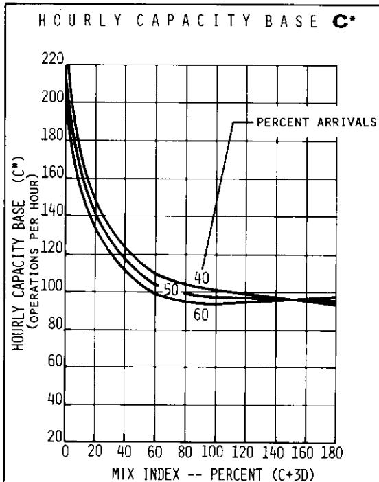
FIGURE 2-38 HOURLY CAPACITY OF RUNWAY USE DIAGRAM NO. 60 FOR VFR CONDITIONS
