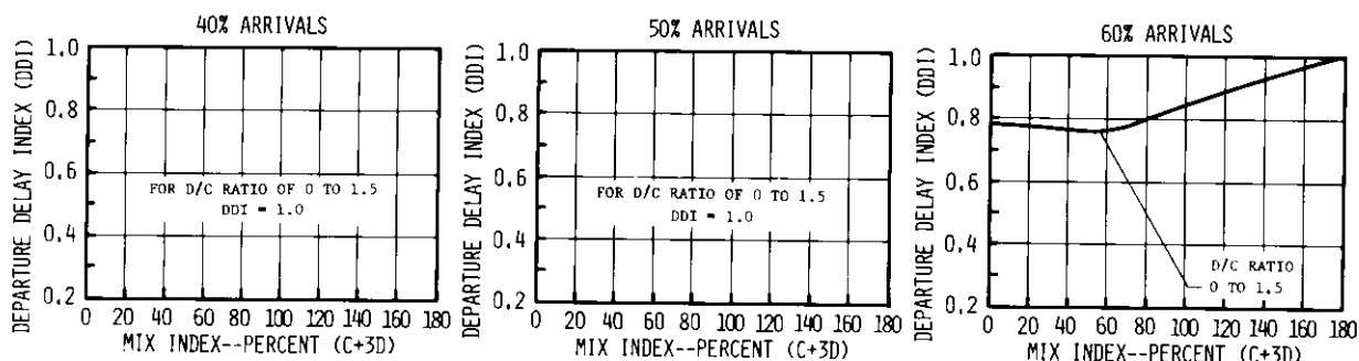
FIGURE 2-75 DELAY INDICES FOR RUNWAY USE DIAGRAMS NOS. 13, 14 FOR VFR CONDITIONS
