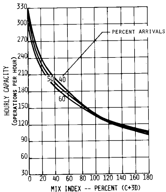
FIGURE A5-4 HOURLY CAPACITY OF RUNWAY USE DIAGRAMS NOS. 30, 31
