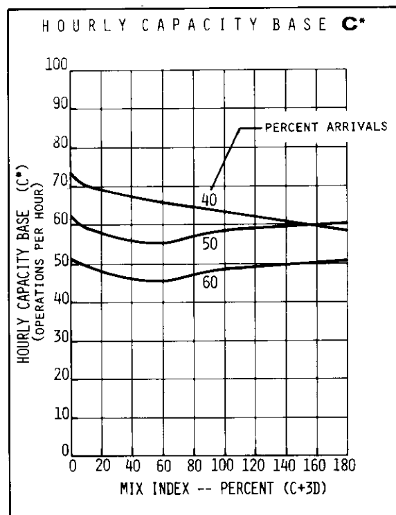
FIGURE 2-60 HOURLY CAPACITY OF RUNWAY USE DIAGRAMS NOS. 45, 51, 57 FOR IFR CONDITIONS
