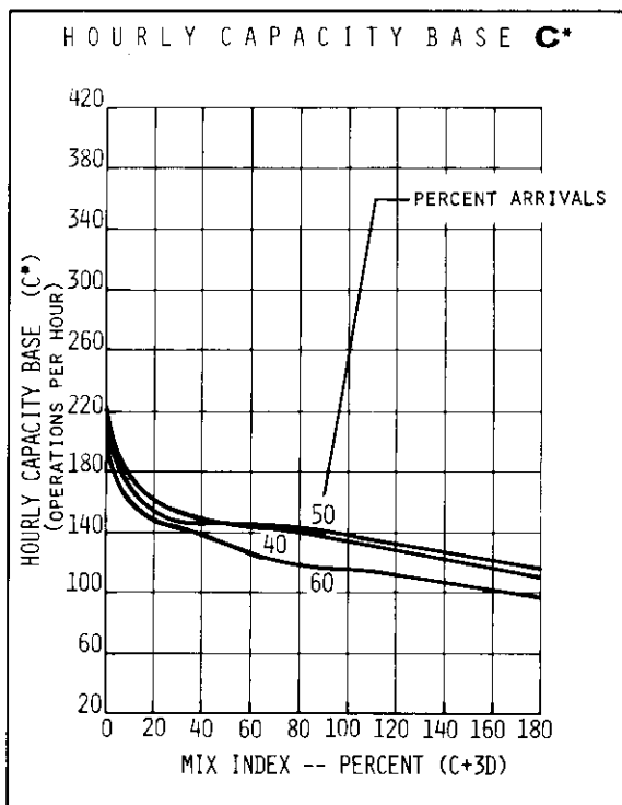
FIGURE 2-34 HOURLY CAPACITY OF RUNWAY USE DIAGRAM NO. 56 FOR VFR CONDITIONS
