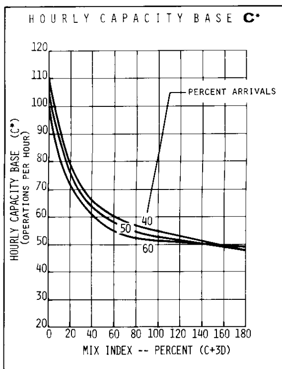
FIGURE 2-32 HOURLY CAPACITY OF RUNWAY USE DIAGRAM NO. 48 FOR VFR CONDITIONS
