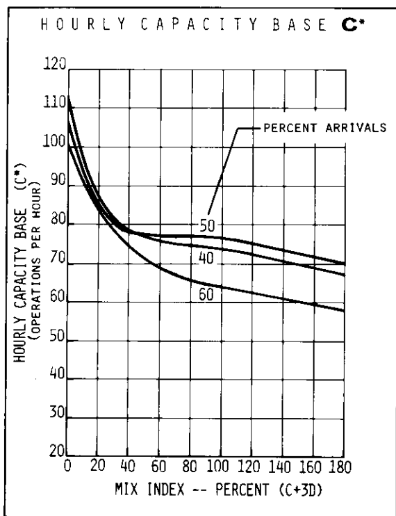
FIGURE 2-30 HOURLY CAPACITY OF RUNWAY USE DIAGRAMS NOS. 46, 52 FOR VFR CONDITIONS
