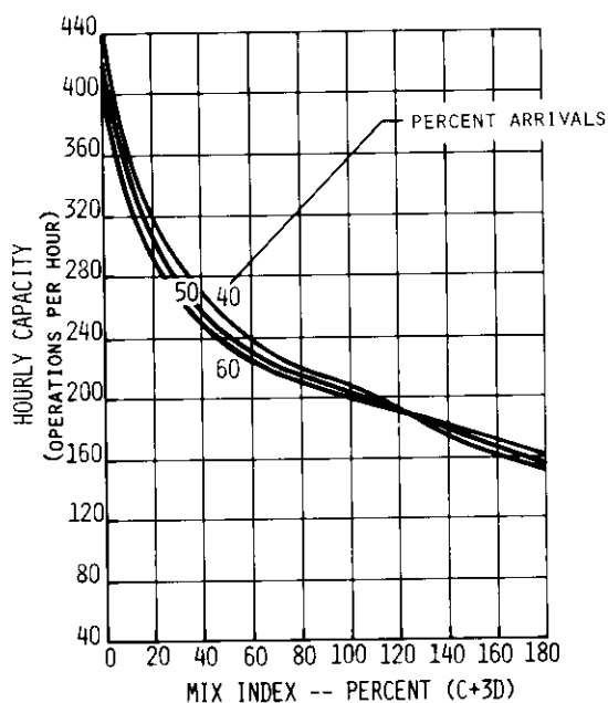
FIGURE A5-5 HOURLY CAPACITY OF RUNWAY USE DIAGRAM NO. 42
