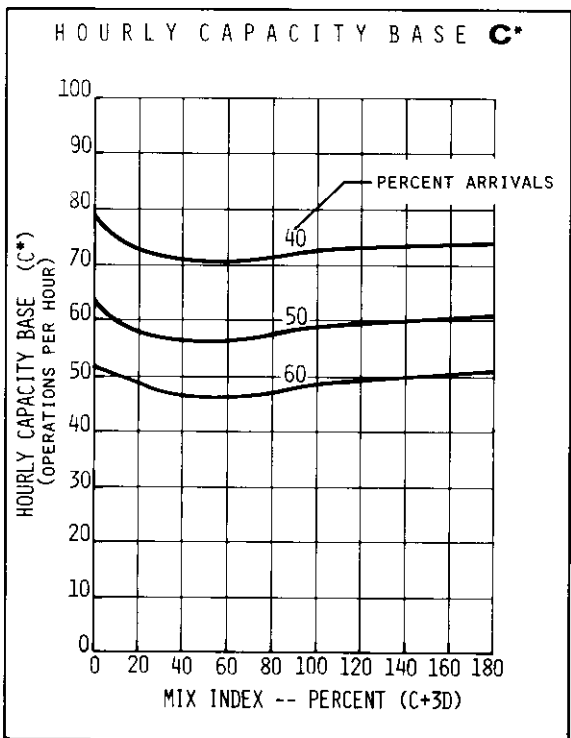
FIGURE 2-58 HOURLY CAPACITY OF RUNWAY USE DIAGRAMS NOS. 43, 49, 55 FOR IFR CONDITIONS
