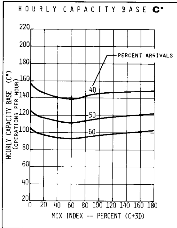
FIGURE 2-57 HOURLY CAPACITY OF RUNWAY USE DIAGRAMS NOS. 32, 33, 34, 35, 37, 38, 39, 40, 41, 42 FOR IFR CONDITIONS
