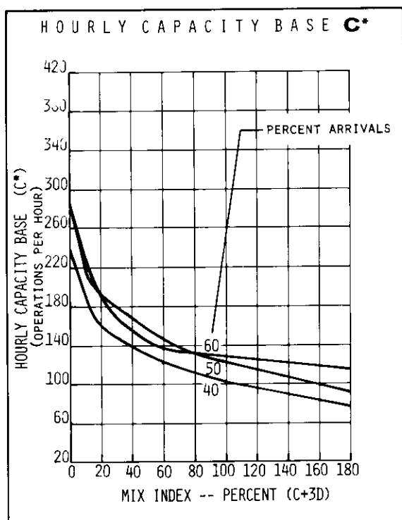
FIGURE 2-11 HOURLY CAPACITY OF RUNWAY USE DIAGRAMS NOS. 13, 14 FOR VFR CONDITIONS
