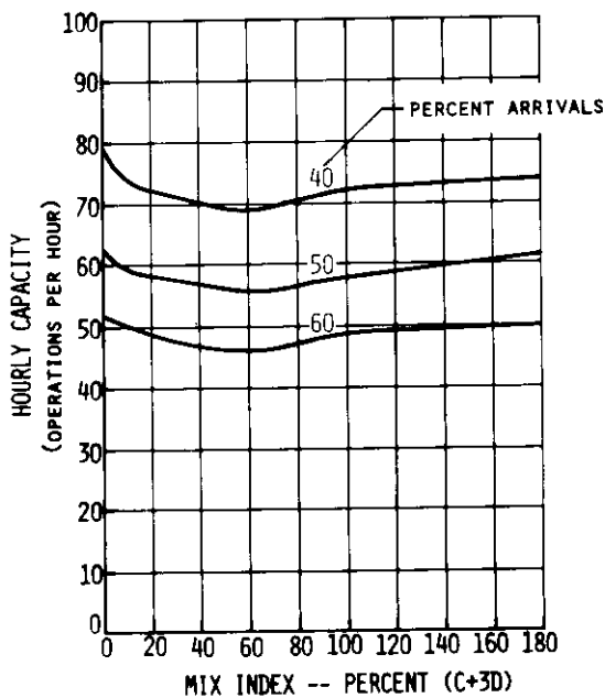
FIGURE A2-4 HOURLY CAPACITY OF RUNWAY USE DIAGRAMS NOS. 2c, 2d
