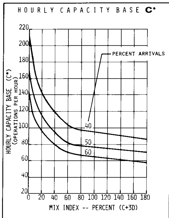
FIGURE 2-5 HOURLY CAPACITY OF RUNWAY USE DIAGRAM NO. 3 FOR VFR CONDITIONS
