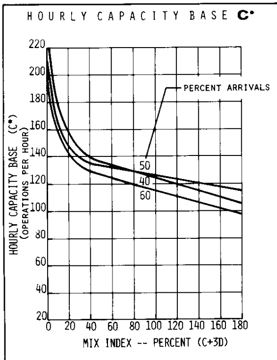
FIGURE 2-35 HOURLY CAPACITY OF RUNWAY USE DIAGRAMS NOS. 57, 63 FOR VFR CONDITIONS
