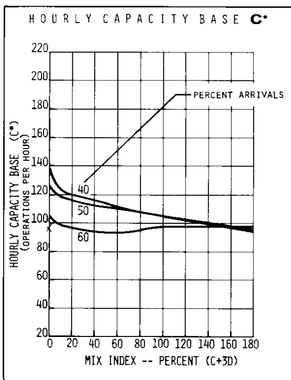
FIGURE 2-50 HOURLY CAPACITY OF RUNWAY USE DIAGRAMS NOS. 12, 71 FOR IFR CONDITIONS
