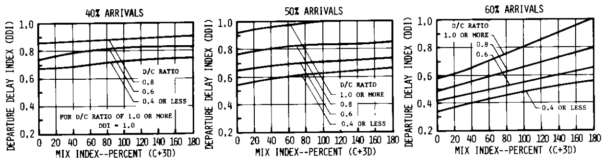
FIGURE 2-96 DELAY INDICES FOR RUNWAY USE DIAGRAMS NOS. 12, 71 FOR IFR CONDITIONS
