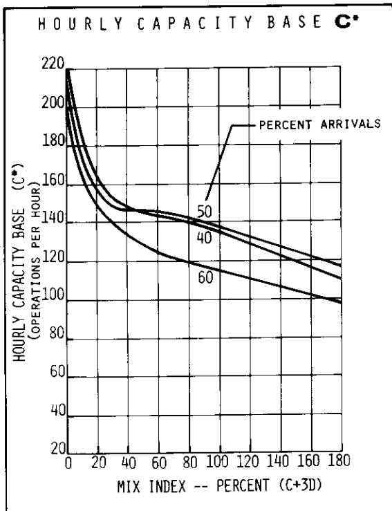
FIGURE 2-39 HOURLY CAPACITY OF RUNWAY USE DIAGRAM NO. 62 FOR VFR CONDITIONS
