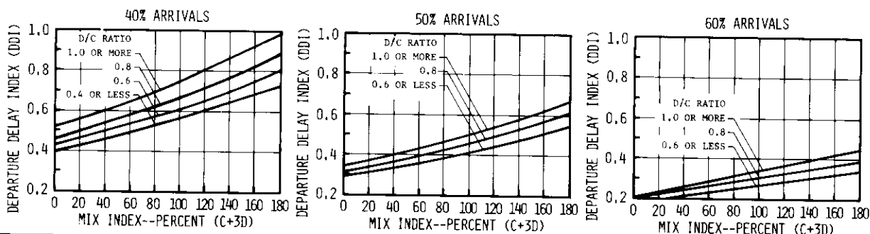
FIGURE 2-95 DELAY INDICES FOR RUNWAY USE DIAGRAMS NOS. 11, 70 FOR IFR CONDITIONS
