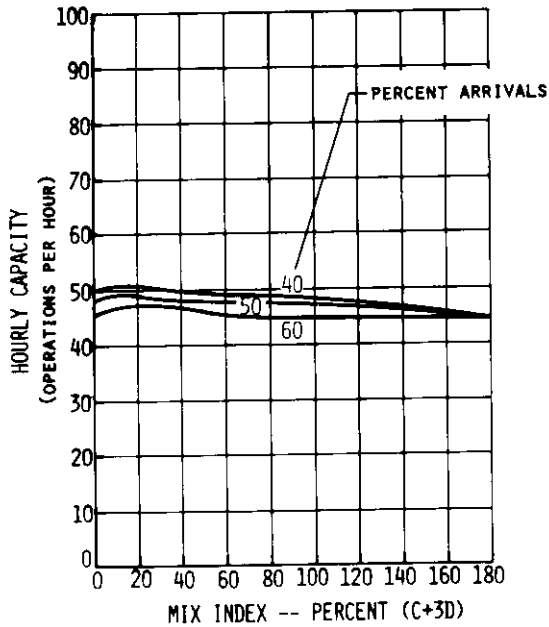
FIGURE A2-2 HOURLY CAPACITY OF RUNWAY USE DIAGRAM NO. 1
