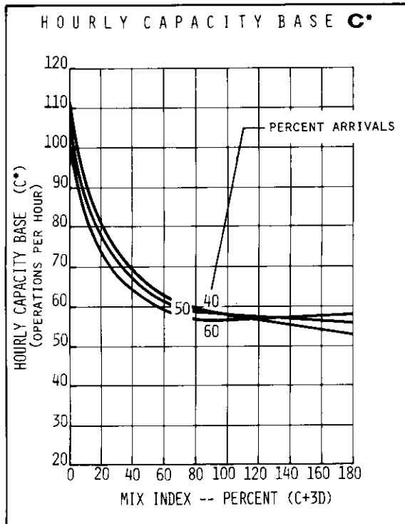
FIGURE 2-31 HOURLY CAPACITY OF RUNWAY USE DIAGRAMS NOS. 47, 53 FOR VFR CONDITIONS
