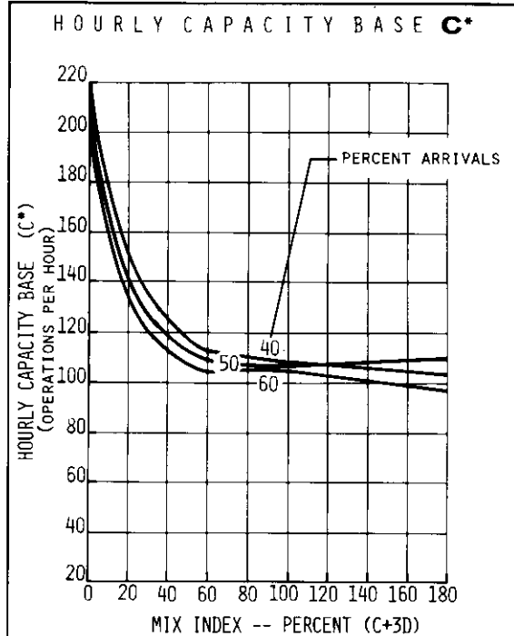
FIGURE 2-37 HOURLY CAPACITY OF RUNWAY USE DIAGRAMS NOS. 59, 65 FOR VFR CONDITIONS
