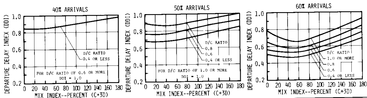
FIGURE 2-76 DELAY INDICES FOR RUNWAY USE DIAGRAMS NOS. 15, 85, 110 FOR VFR CONDITIONS
