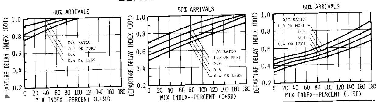
FIGURE 2-92 DELAY INDICES FOR RUNWAY USE DIAGRAM NO. 7 FOR IFR CONDITIONS
