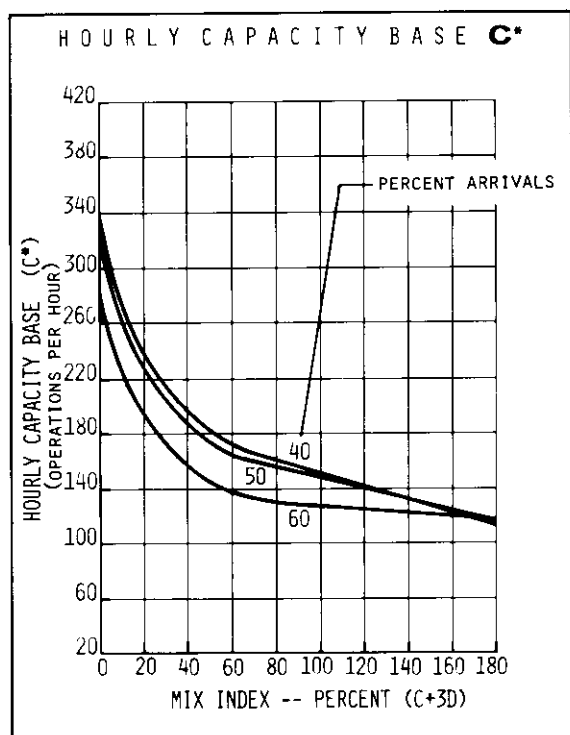
FIGURE 2-12 HOURLY CAPACITY OF RUNWAY USE DIAGRAMS NOS. 15, 85, 110 FOR VFR CONDITIONS
