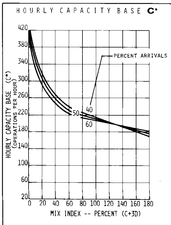
FIGURE 2-26 HOURLY CAPACITY OF RUNWAY USE DIAGRAM NO. 42 FOR VFR CONDITIONS
