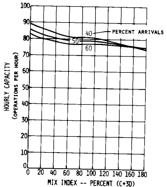
FIGURE A2-9 HOURLY CAPACITY OF RUNWAY USE DIAGRAM NO. 8
