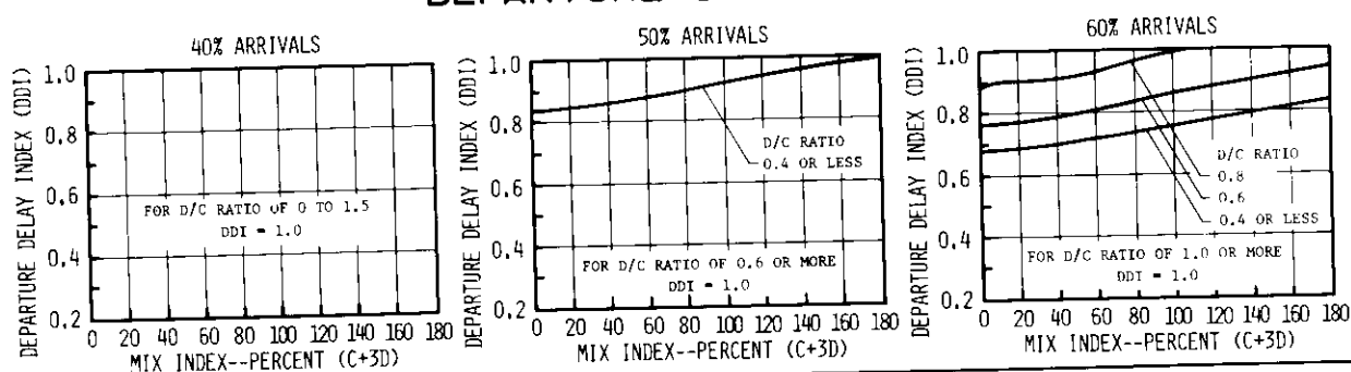
FIGURE 2-93 DELAY INDICES FOR RUNWAY USE DIAGRAM NO. 8 FOR IFR CONDITIONS
