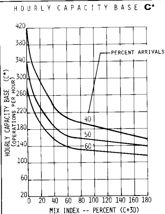
FIGURE 2-20 HOURLY CAPACITY OF RUNWAY USE DIAGRAMS NOS. 32, 33 FOR VFR CONDITIONS
