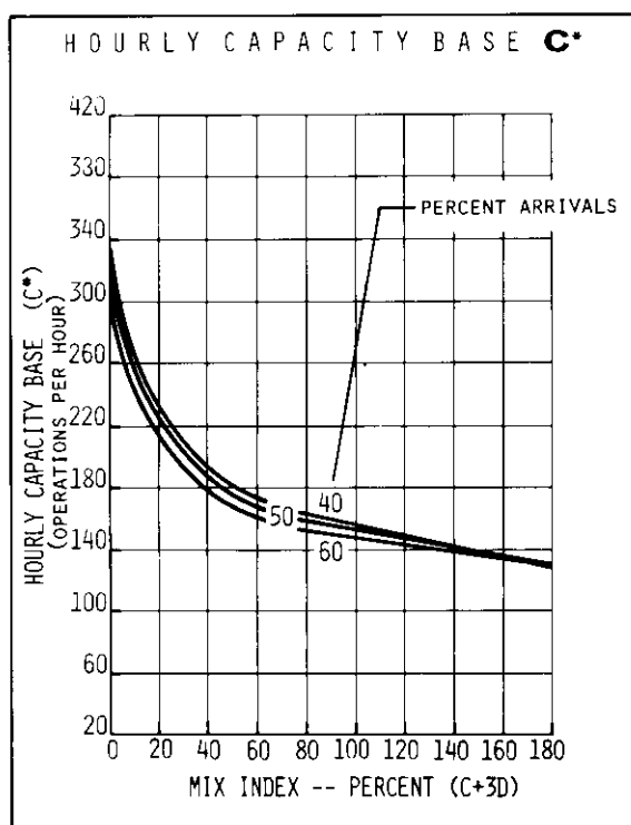
FIGURE 2-16 HOURLY CAPACITY OF RUNWAY USE DIAGRAM NOS. 24, 25 FOR VFR CONDITIONS
