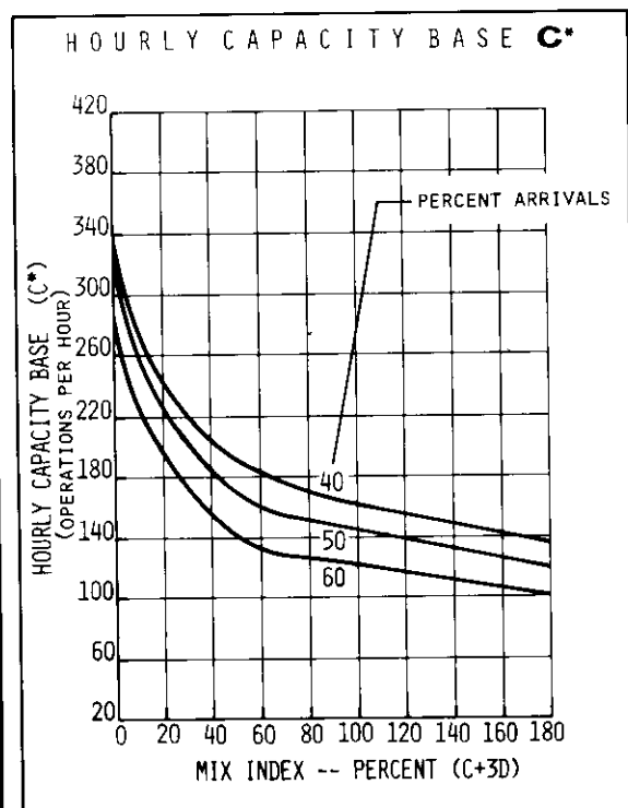
FIGURE 2-40 HOURLY CAPACITY OF RUNWAY USE DIAGRAMS NOS. 86, 87, 88, 89, 90, 111, 112, 113, 114, 115 FOR VFR CONDITIONS
