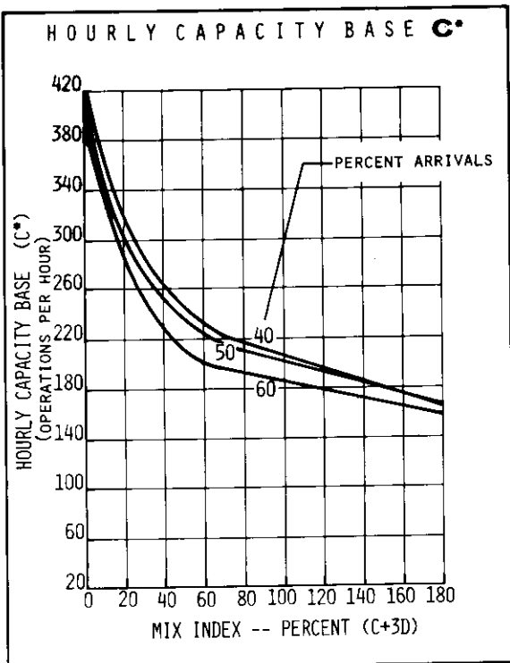
FIGURE 2-23 HOURLY CAPACITY OF RUNWAY USE DIAGRAM NO. 39 FOR VFR CONDITIONS
