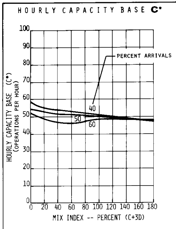
FIGURE 2-63 HOURLY CAPACITY OF RUNWAY USE DIAGRAM NOS. 48, 60 FOR IFR CONDITIONS
