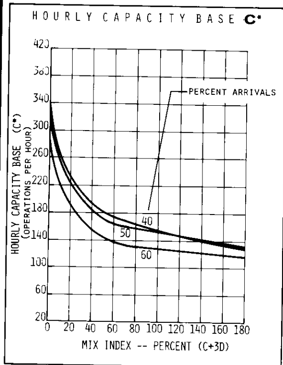
FIGURE 2-13 HOURLY CAPACITY OF RUNWAY USE DIAGRAMS NOS. 16, 17, 19, 20 FOR VFR CONDITIONS
