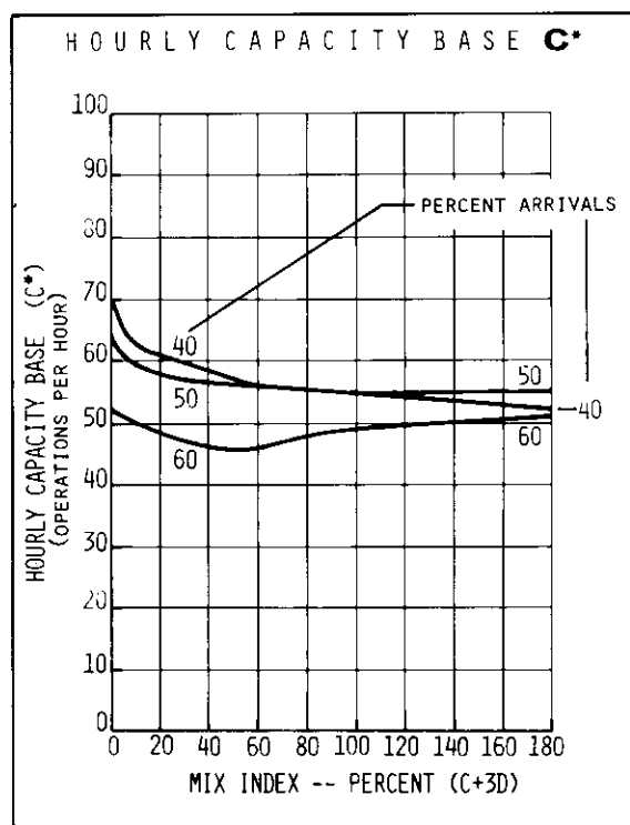
FIGURE 2-64 HOURLY CAPACITY OF RUNWAY USE DIAGRAM NO. 53 FOR IFR CONDITIONS
