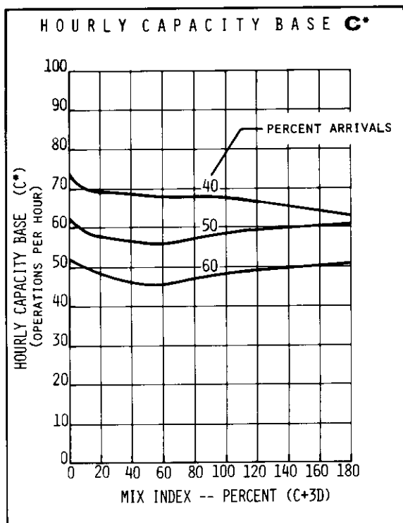
FIGURE 2-59 HOURLY CAPACITY OF RUNWAY USE DIAGRAMS NOS. 44, 50, 56 FOR IFR CONDITIONS
