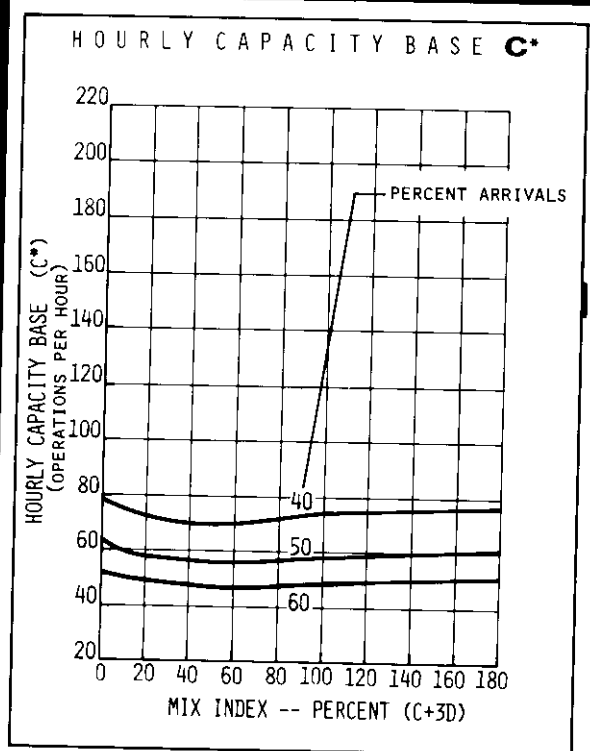
FIGURE 2-54 HOURLY CAPACITY OF RUNWAY USE DIAGRAMS NOS. 18, 21, 80, 82, 86, 88, 94, 105, 107, 111, 113, 119 FOR IFR CONDITIONS
