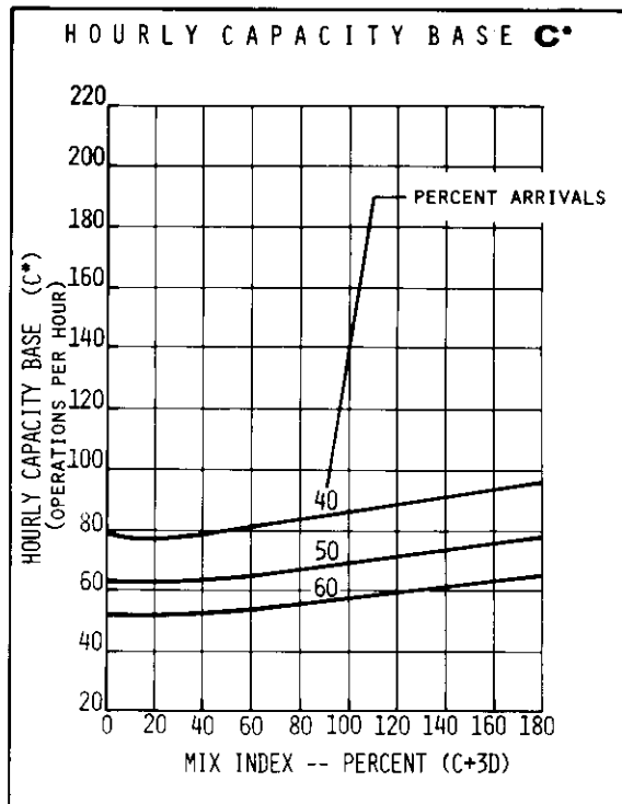
FIGURE 2-49 HOURLY CAPACITY OF RUNWAY USE DIAGRAMS NOS. 11, 70 FOR IFR CONDITIONS
