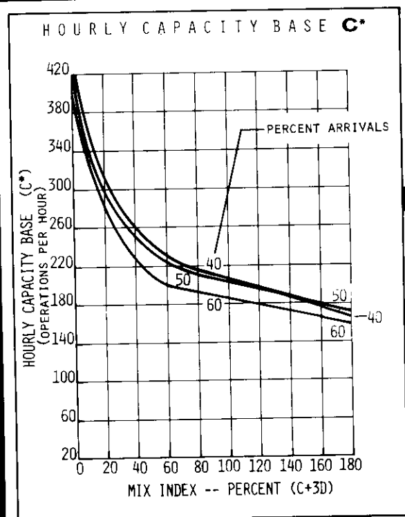
FIGURE 2-24 HOURLY CAPACITY OF RUNWAY USE DIAGRAM NO. 40 FOR VFR CONDITIONS
