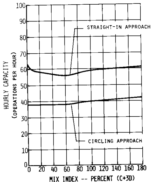
FIGURE A3-3A HOURLY CAPACITY IN RADAR ENVIRONMENT
