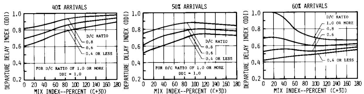
FIGURE 2-85 DELAY INDICES FOR RUNWAY USE DIAGRAMS NOS. 44, 45, 46, 50, 51, 52, 56, 57, 58, 62, 63, 64 FOR VFR CONDITIONS
