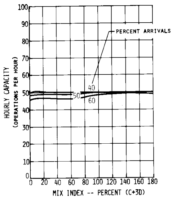
FIGURE A2-14 HOURLY CAPACITY OF RUNWAY USE DIAGRAMS NOS. 43b, 49b
