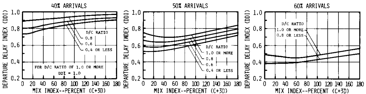
FIGURE 2-99 DELAY INDICES FOR RUNWAY USE DIAGRAMS NOS. 17, 20, 25, 31, 36, 44, 45, 46, 50, 51, 52, 56, 57, 58 FOR IFR CONDITIONS
