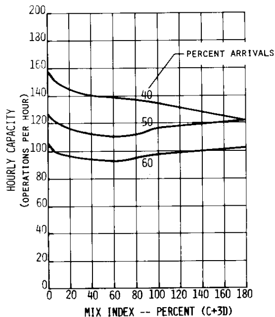
FIGURE A5-10 HOURLY CAPACITY OF RUNWAY USE DIAGRAM NO. 42
