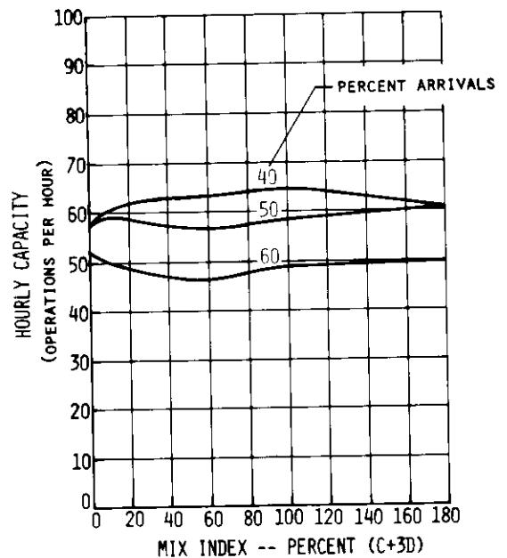
FIGURE A2-13 HOURLY CAPACITY OF RUNWAY USE DIAGRAMS NOS. 43a, 49a
