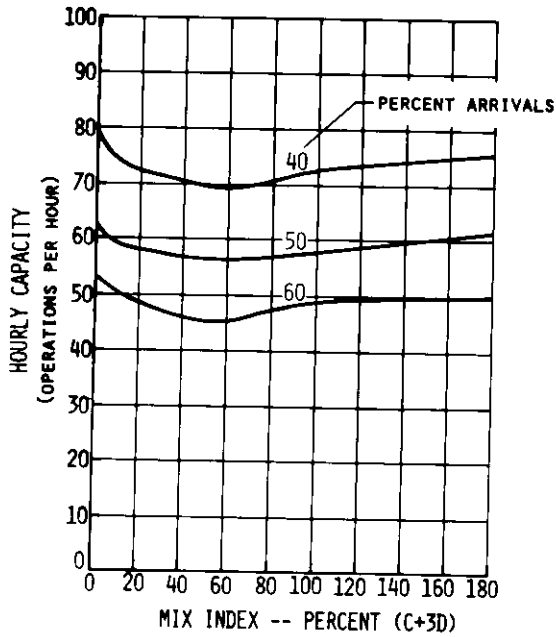
FIGURE A2-6 HOURLY CAPACITY OF RUNWAY USE DIAGRAM NO. 5
