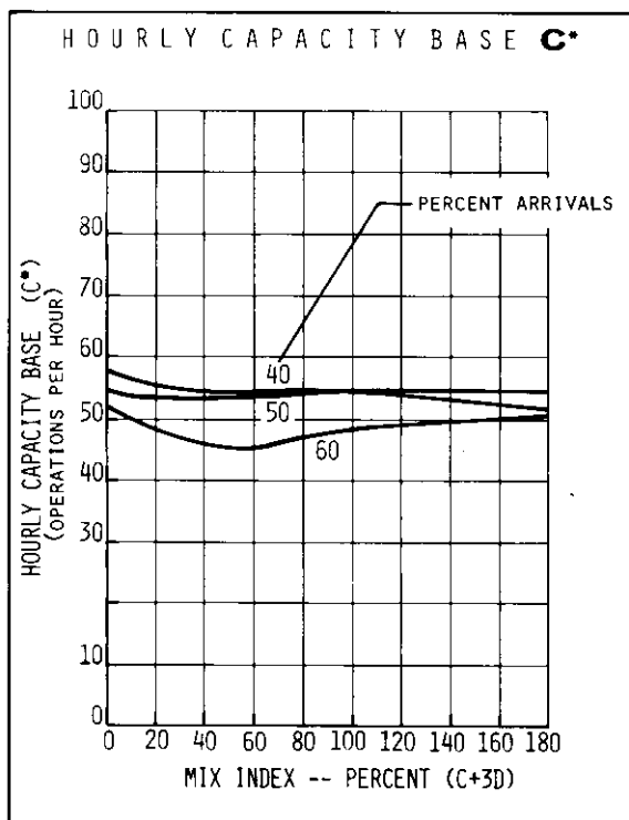
FIGURE 2-62 HOURLY CAPACITY OF RUNWAY USE DIAGRAMS NOS. 47, 59 FOR IFR CONDITIONS
