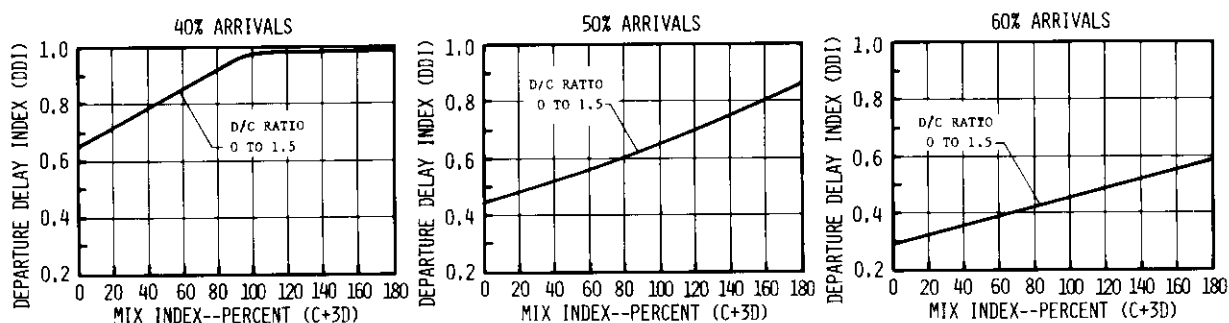
FIGURE 2-97 DELAY INDICES FOR RUNWAY USE DIAGRAMS NOS. 13, 15, 16, 23, 24, 26, 27 FOR IFR CONDITIONS
