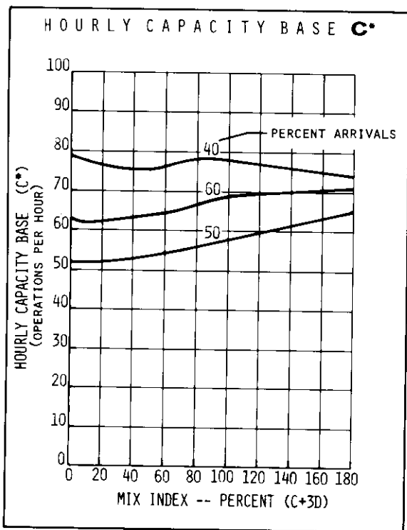
FIGURE 2-46 HOURLY CAPACITY OF RUNWAY USE DIAGRAM NO. 7 FOR IFR CONDITIONS
