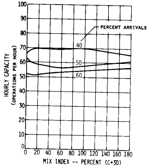
FIGURE A2-7 HOURLY CAPACITY OF RUNWAY USE DIAGRAM NO. 7a
