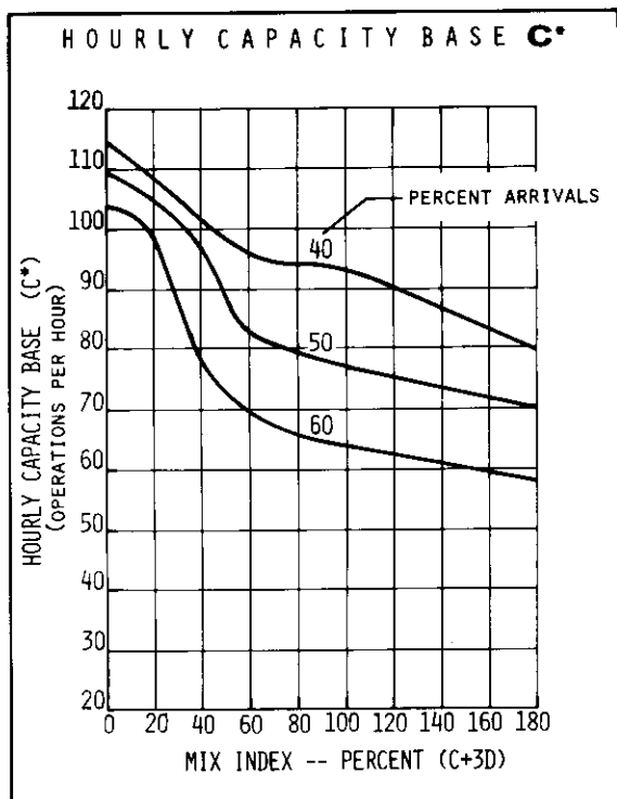
FIGURE 2-27 HOURLY CAPACITY OF RUNWAY USE DIAGRAMS NOS. 43, 49 FOR VFR CONDITIONS
