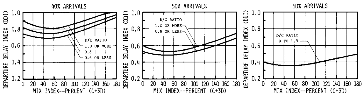
FIGURE 2-81 DELAY INDICES FOR RUNWAY USE DIAGRAMS NOS. 34, 35 FOR VFR CONDITIONS
