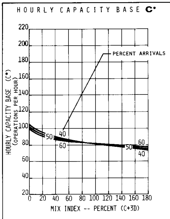
FIGURE 2-47 HOURLY CAPACITY OF RUNWAY USE DIAGRAM NO. 8 FOR IFR CONDITIONS
