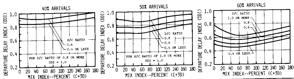
FIGURE 2-77 DELAY INDICES FOR RUNWAY USE DIAGRAMS NOS. 16, 17, 18, 19, 20, 21, 22, 80, 81, 82, 83, 84, 105, 106, 107, 108, 109 FOR VFR CONDITIONS
