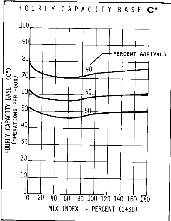
FIGURE 2-45 HOURLY CAPACITY OF RUNWAY USE DIAGRAMS NOS. 5, 75, 77, 78, 100, 102, 103 FOR IFR CONDITIONS
