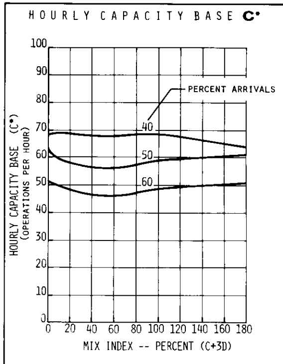
FIGURE 2-61 HOURLY CAPACITY OF RUNWAY USE DIAGRAMS NOS. 46, 52, 58 FOR IFR CONDITIONS
