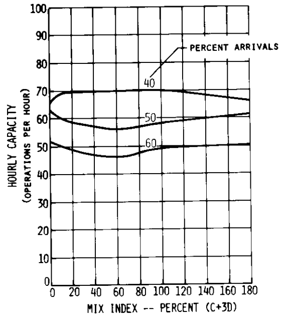
FIGURE A2-3 HOURLY CAPACITY OF RUNWAY USE DIAG. NOS. 2a, 2b, 3, 6, 9
