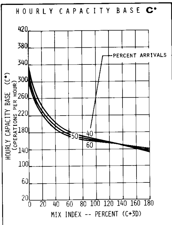
FIGURE 2-19 HOURLY CAPACITY OF RUNWAY USE DIAGRAMS NOS. 30, 31 FOR VFR CONDITIONS
