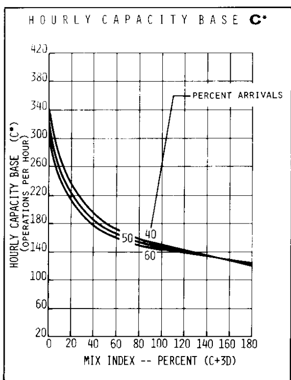
FIGURE 2-18 HOURLY CAPACITY OF RUNWAY USE DIAGRAM NO. 29 FOR VFR CONDITIONS
