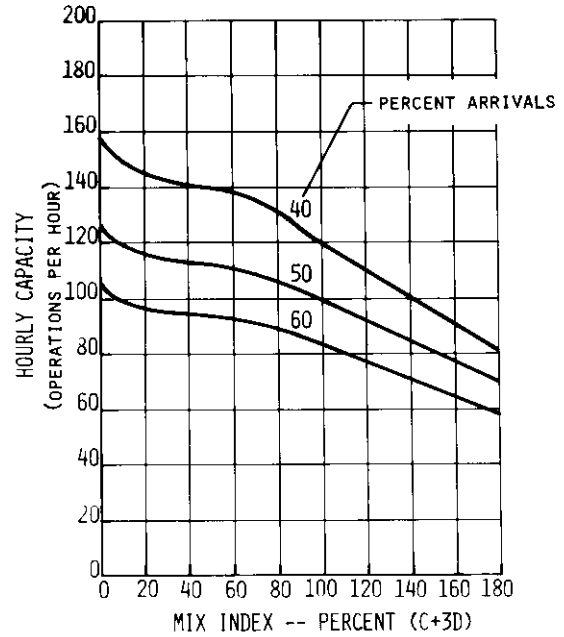
FIGURE A5-9 HOURLY CAPACITY OF RUNWAY USE DIAGRAM NO. 31
