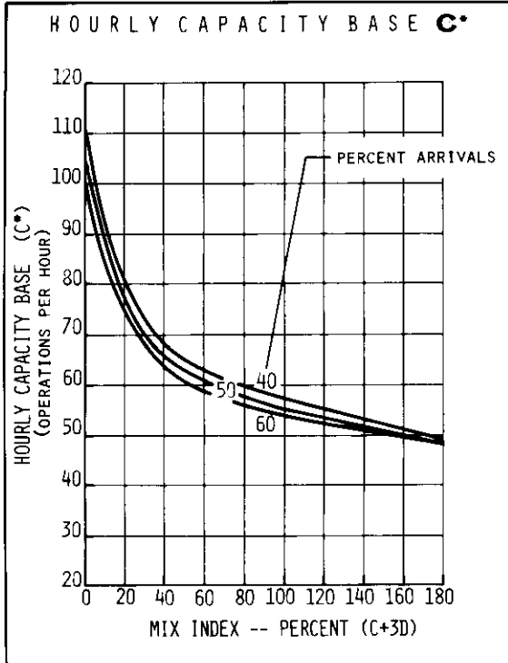
FIGURE 2-3 HOURLY CAPACITY OF RUNWAY USE DIAGRAM NOS. 1, 54 FOR VFR CONDITIONS
