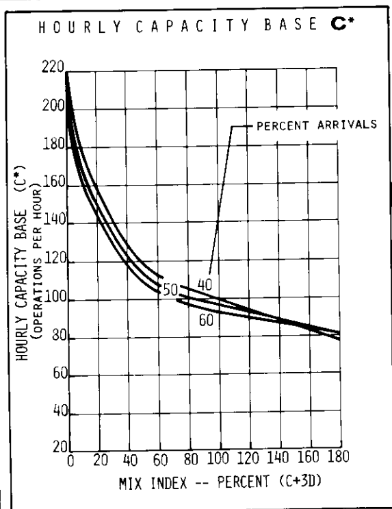
FIGURE 2-7 HOURLY CAPACITY OF RUNWAY USE DIAGRAM NO. 6 FOR VFR CONDITIONS
