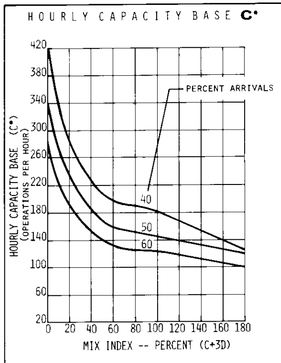
FIGURE 2-41 HOURLY CAPACITY OF RUNWAY USE DIAGRAMS NOS. 92, 93, 117, 118, 122 FOR VFR CONDITIONS
