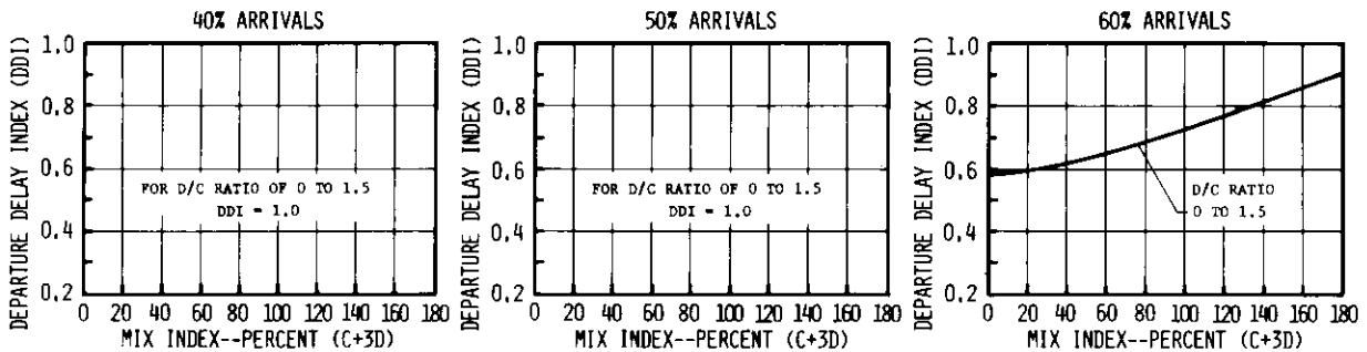
FIGURE 2-98 DELAY INDICES FOR RUNWAY USE DIAGRAMS NOS. 14, 28 FOR IFR CONDITIONS
