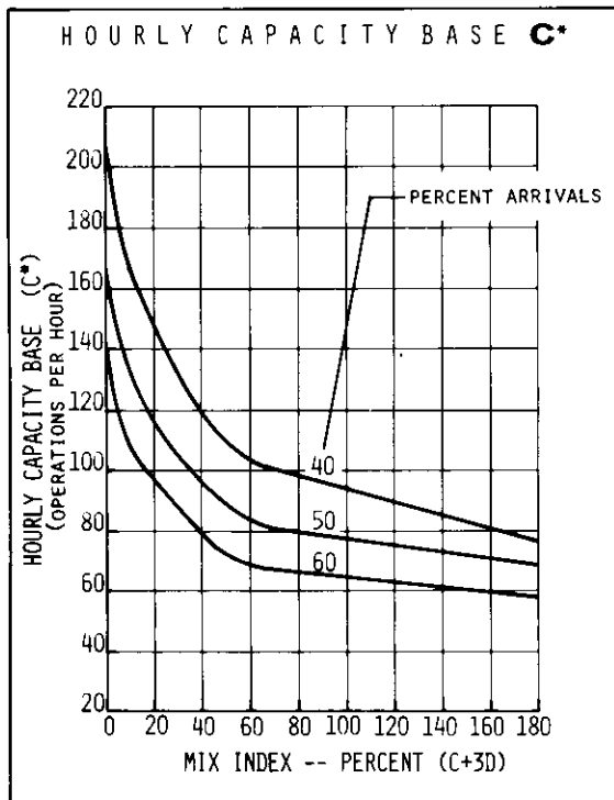
FIGURE 2-4 HOURLY CAPACITY OF RUNWAY USE DIAGRAM NOS. 2, 67, 72, 73, 97, 98 FOR VFR CONDITIONS
