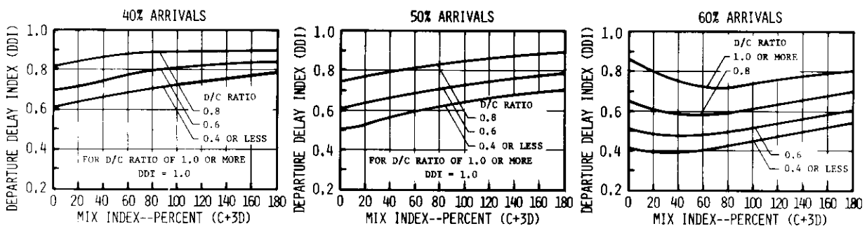
FIGURE 2-102 DELAY INDICES FOR RUNWAY USE DIAGRAMS NOS. 47, 48, 59, 60 FOR IFR CONDITIONS
