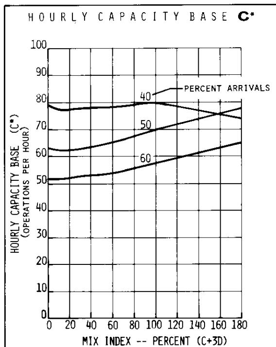
FIGURE 2-48 HOURLY CAPACITY OF RUNWAY USE DIAGRAMS NOS. 10, 29, 69 FOR IFR CONDITIONS
