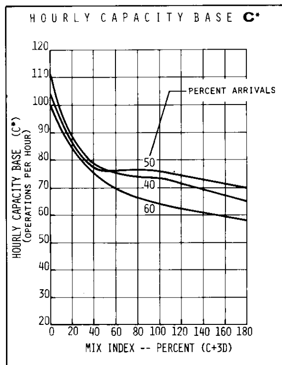
FIGURE 2-28 HOURLY CAPACITY OF RUNWAY USE DIAGRAMS NOS. 44, 50 FOR VFR CONDITIONS
