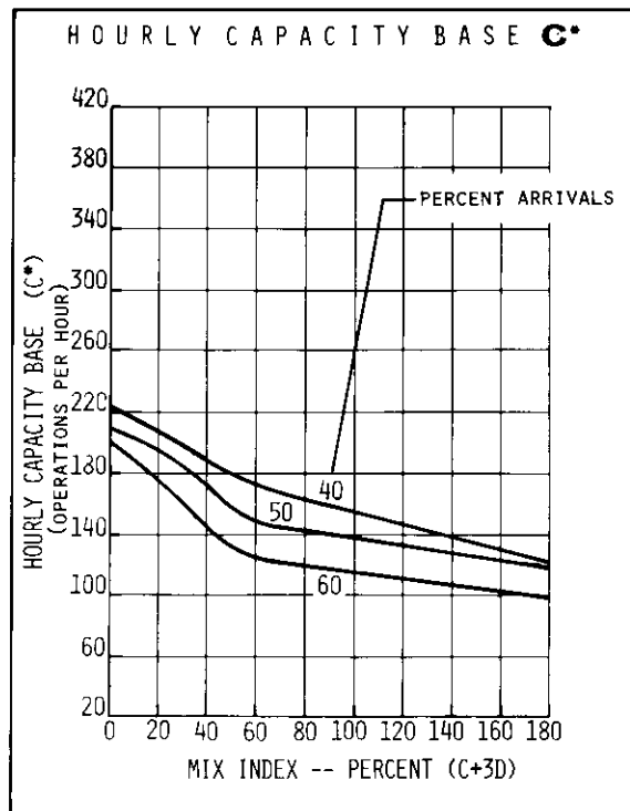
FIGURE 2-33 HOURLY CAPACITY OF RUNWAY USE DIAGRAMS NOS. 55, 61 FOR VFR CONDITIONS
