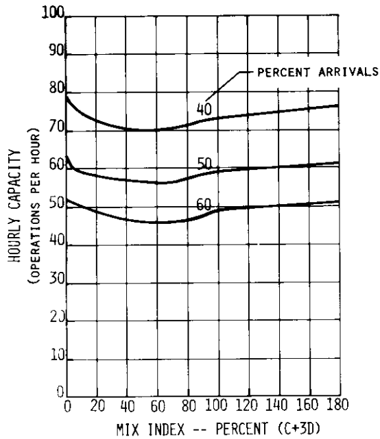
FIGURE A5-8 HOURLY CAPACITY OF RUNWAY USE DIAGRAM NO. 30
