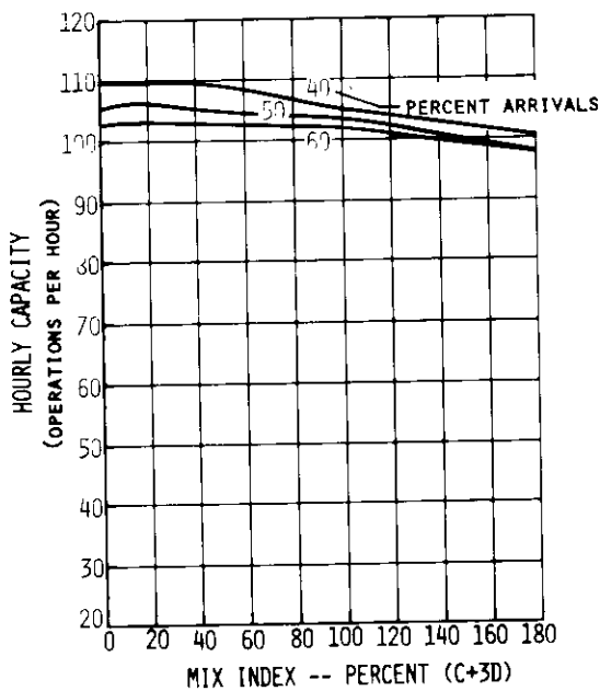
FIGURE A2-12 HOURLY CAPACITY OF RUNWAY USE DIAGRAM NO. 12
