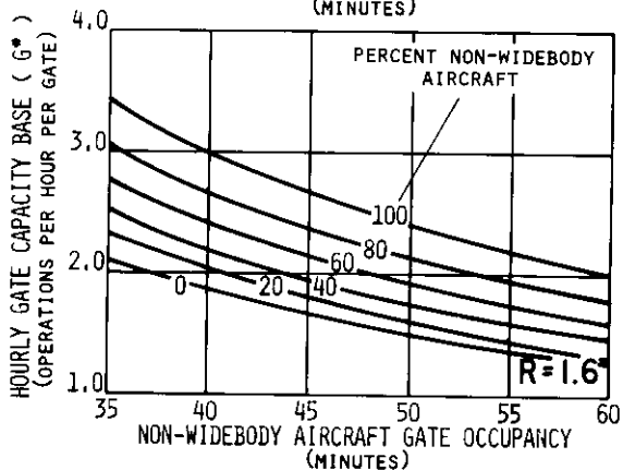
FIGURE 2-67 HOURLY CAPACITY OF GATES
