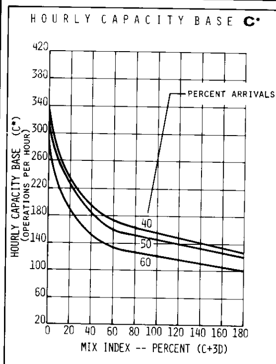
FIGURE 2-14 HOURLY CAPACITY OF RUNWAY USE DIAGRAMS NOS. 18, 21, 22, 80, 81, 82, 83, 84, 105, 106, 107, 108, 109 FOR VFR CONDITIONS
