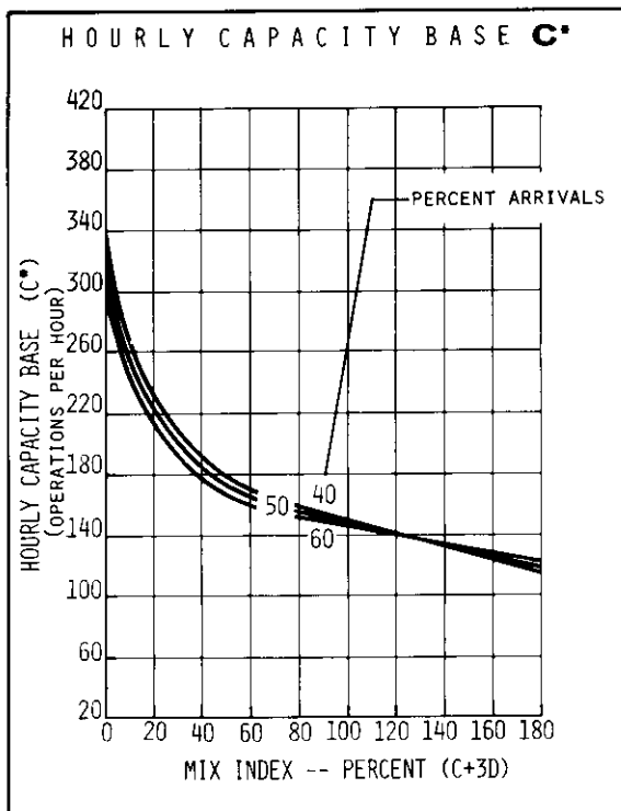
FIGURE 2-15 HOURLY CAPACITY OF RUNWAY USE DIAGRAM NOS. 23, 26 FOR VFR CONDITIONS
