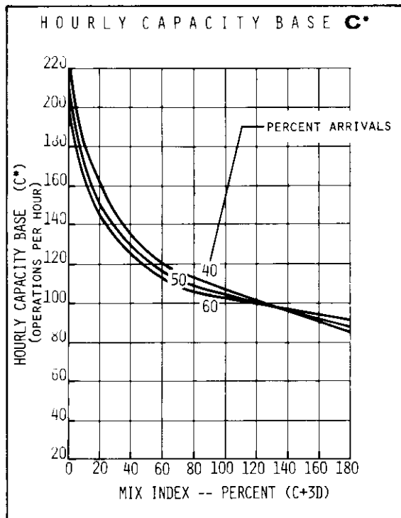
FIGURE 2-9 HOURLY CAPACITY OF RUNWAY USE DIAGRAMS NOS. 9, 66, 68 FOR VFR CONDITIONS
