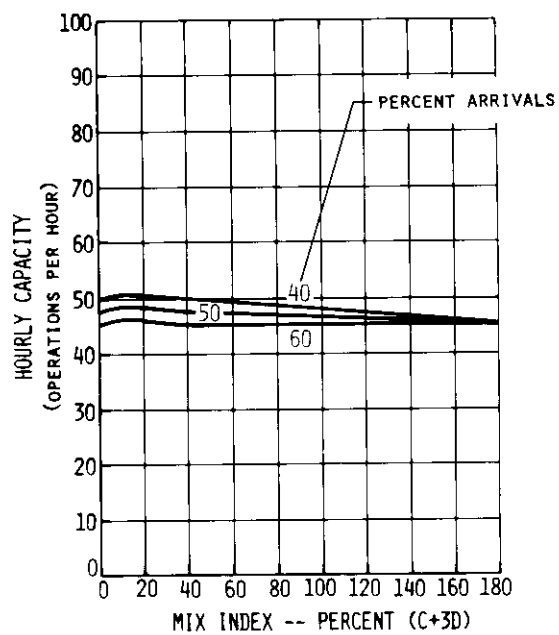
FIGURE A2-15 HOURLY CAPACITY OF RUNWAY USE DIAGRAMS NOS. 43c, 49c
