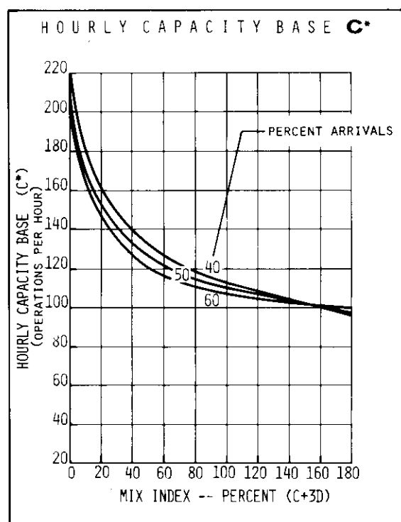
FIGURE 2-10 HOURLY CAPACITY OF RUNWAY USE DIAGRAMS NOS. 10, 11, 12, 69, 70, 71 FOR VFR CONDITIONS
