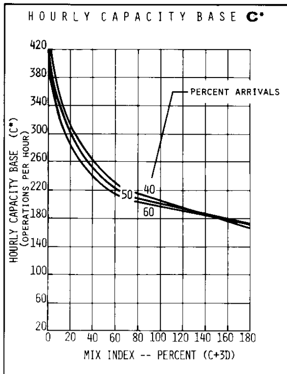
FIGURE 2-25 HOURLY CAPACITY OF RUNWAY USE DIAGRAM NO. 41 FOR VFR CONDITIONS
