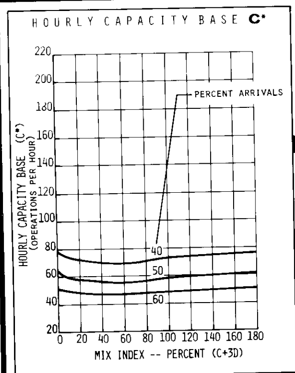
FIGURE 2-56 HOURLY CAPACITY OF RUNWAY USE DIAGRAMS NOS. 22, 81, 83, 84, 87, 89, 90, 95, 96, 106, 108, 109, 112, 114, 115, 120, 121 FOR IFR CONDITIONS
