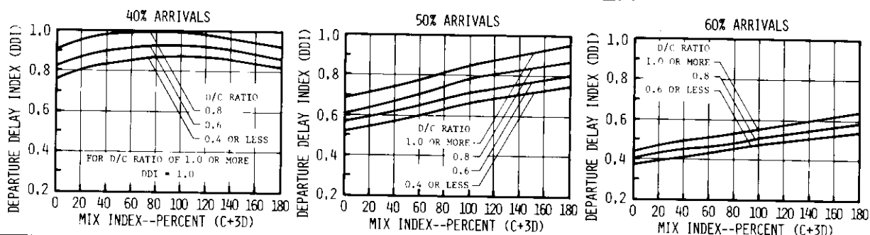
FIGURE 2-94 DELAY INDICES FOR RUNWAY USE DIAGRAMS NOS. 10, 29, 69 FOR IFR CONDITIONS
