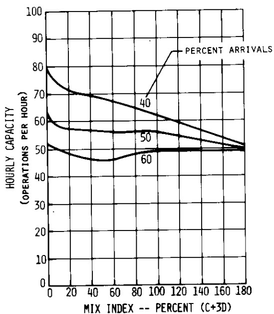
FIGURE A5-6 HOURLY CAPACITY OF RUNWAY USE DIAGRAMS NO. 9, 10, 11
