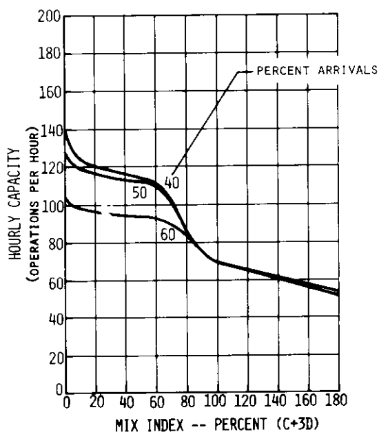
FIGURE A5-7 HOURLY CAPACITY OF RUNWAY USE DIAGRAM NO. 12
