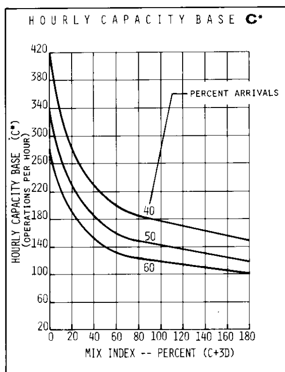
FIGURE 2-42 HOURLY CAPACITY OF RUNWAY USE DIAGRAMS NOS. 94, 95, 96, 119, 120, 121 FOR VFR CONDITIONS
