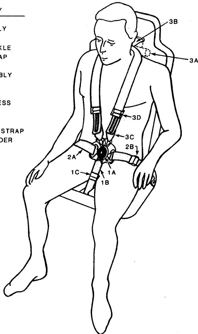
FIGURE 23. BASIC AIRCREW RESTRAINT SYSTEM. (REFERENCE 15)
