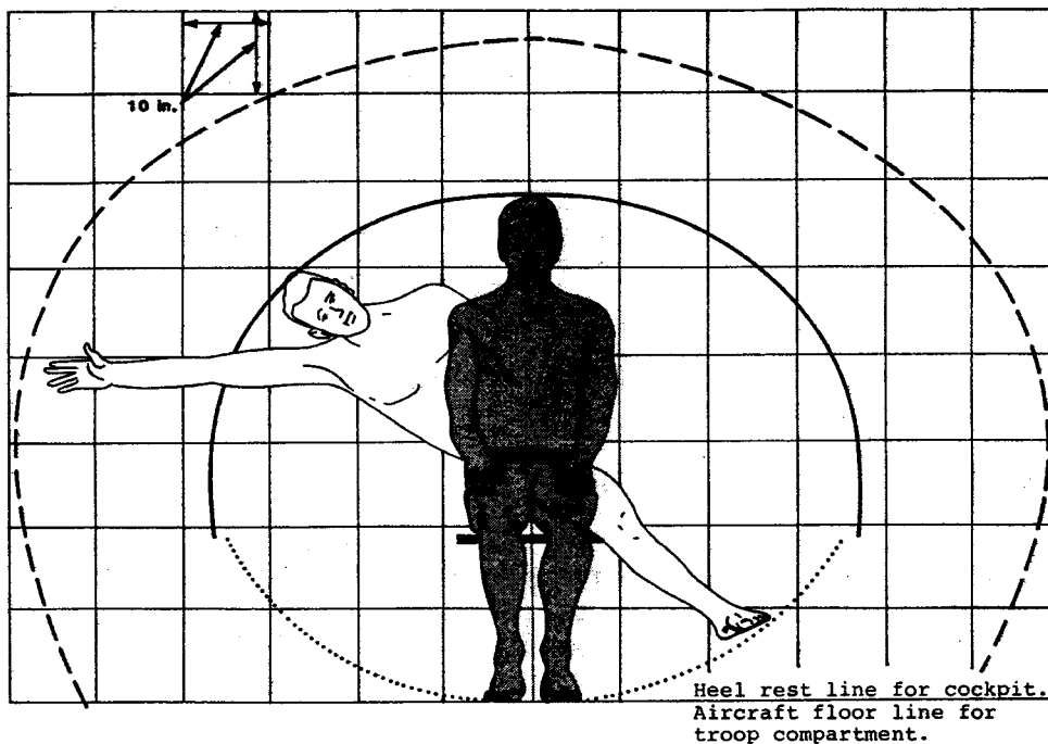
FIGURE 48. LAP-BELT-ONLY EXTREMITY STRIKE ENVELOPE - FRONT VIEW.
