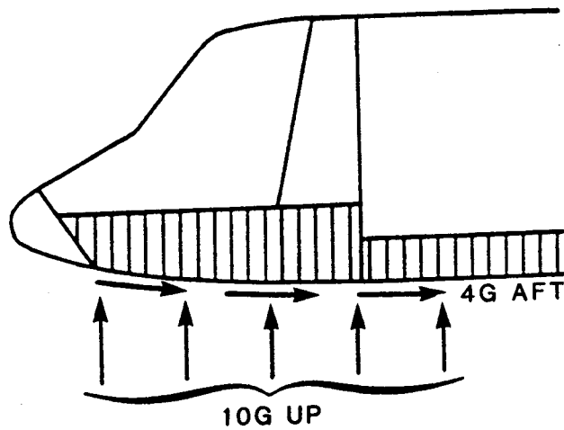
FIGURE 44. DESIGN CRITERIA FOR PLOWING CONDITION.
