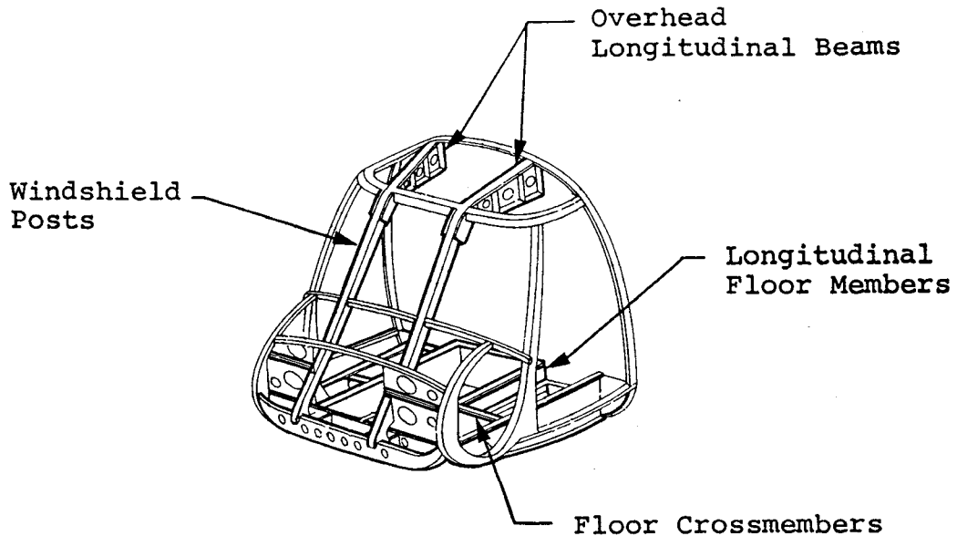
FIGURE 50. LONGITUDINAL IMPACT AND BLADE STRIKE PROTECTION IN NOSE SECTION. THE FIGURE DELINEATES THOSE MEMBERS REQUIRING CAREFUL DESIGN CONSIDERATION.
