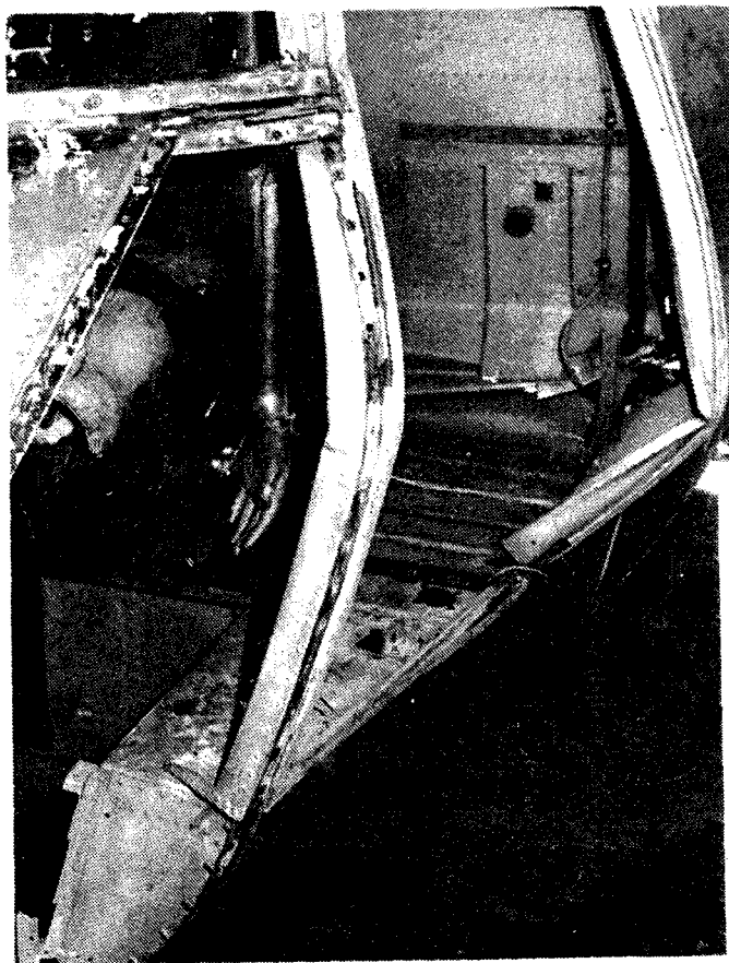
FIGURE 20. TYPICAL FRAME FAILURE AWAY FROM OCCUPIED SPACE IN THE COCKPIT AREA OF A MEDIUM CARGO HELICOPTER FOLLOWING VERTICAL IMPACT.
