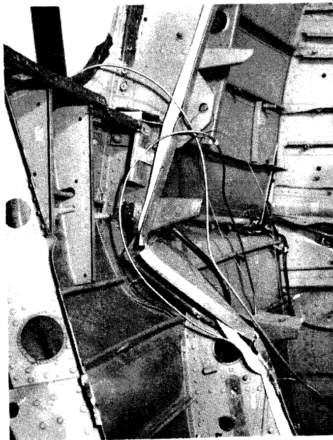
FIGURE 21. TYPICAL FRAME FAILURE AWAY FROM OCCUPIED SPACE IN THE CABIN AREA OF A MEDIUM CARGO HELICOPTER FOLLOWING VERTICAL IMPACT.
