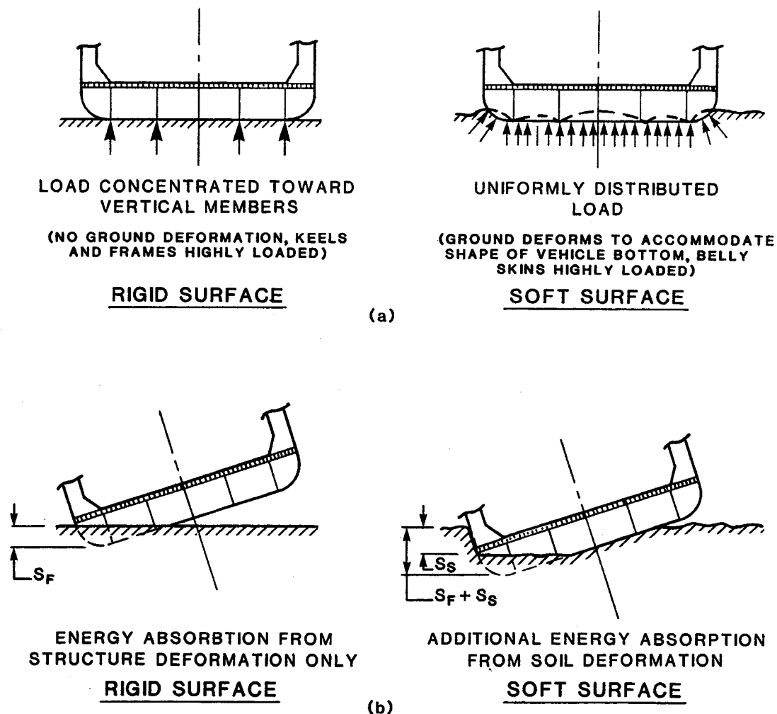
FIGURE 96. LOAD DISTRIBUTIONS ON HARD AND SOFT SURFACES.
