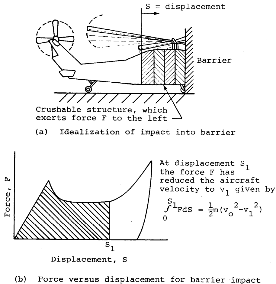
FIGURE 83. ILLUSTRATION OF IMPACT REDUCING AIRCRAFT KINETIC ENERGY.
