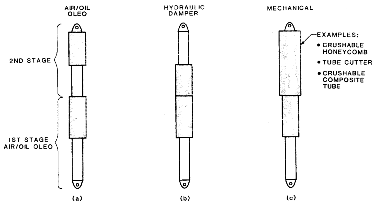
FIGURE 78. TWO-STAGE SHOCK STRUT CONCEPTS.
