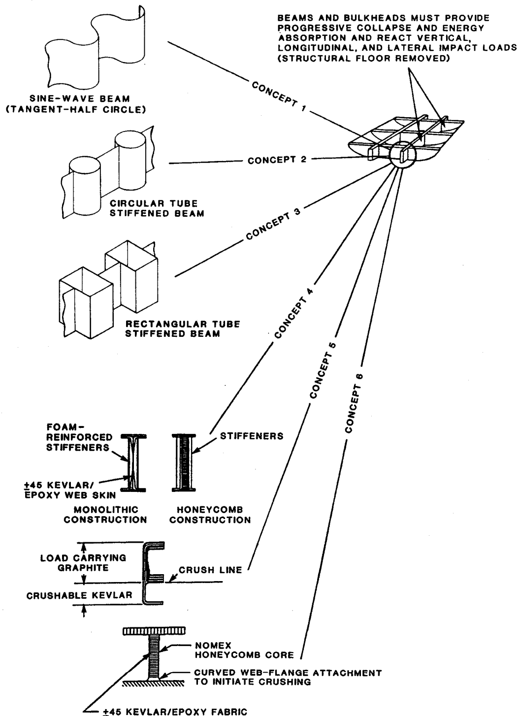
FIGURE 38. ENERGY ABSORPTION CONCEPTS - BEAMS AND BULKHEAD (VERTICAL IMPACT). (FROM REFERENCES 27, 29, 30, 44, AND 50)
