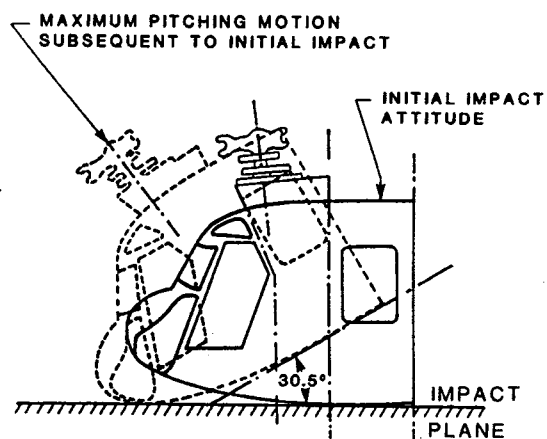
b. INITIAL IMPACT ATTITUDE AND SUBSEQUENT NOSE-DOWN PITCHING MOTION IN MEDIUM CARGO HELICOPTER NOSE SECTION DROP TEST
