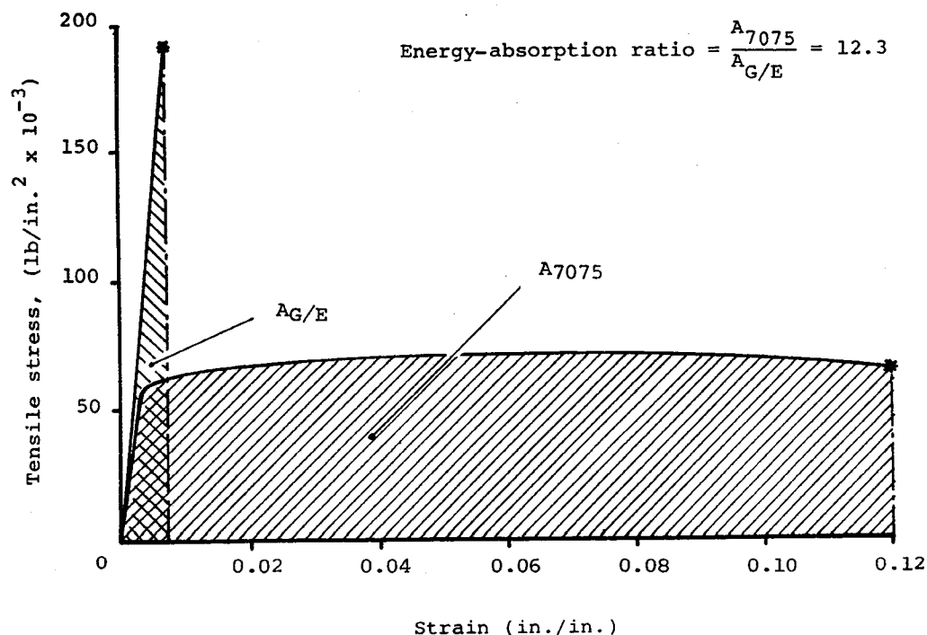
FIGURE 28. STRESS-STRAIN RELATIONSHIP FOR ALUMINUM ALLOY (7075) AND 0-DEGREES GRAPHITE/EPOXY COMPOSITE.
