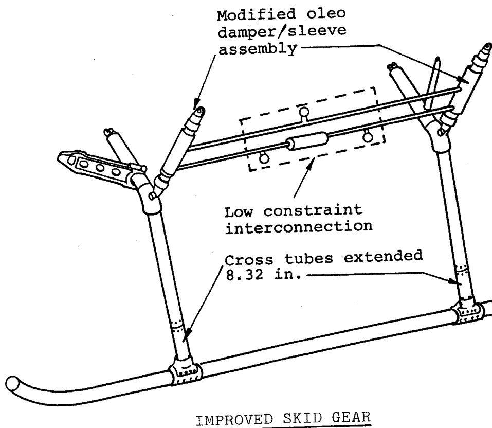
FIGURE 74. HELICOPTER SKID GEAR AND IMPROVED, PITCH-INTERCONNECTED CONCEPTS.
