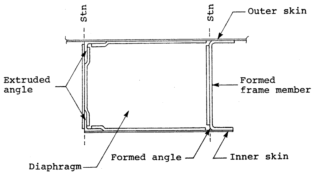
FIGURE 54. EXAMPLES OF CLOSED BOX-BEAM FRAME SECTIONS.
