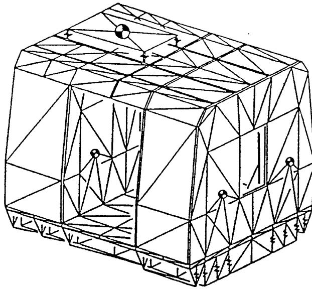
a. FINITE ELEMENT MODEL OF THE COMPOSITE CABIN SECTION
