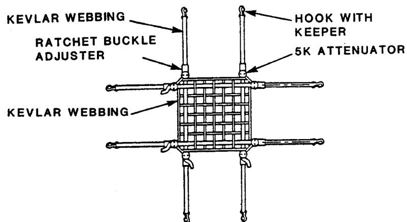
FIGURE 66. CRASH-RESISTANT BARRIER NET. (FROM REFERENCE 81)
