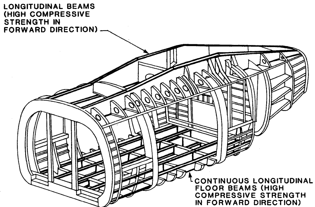
FIGURE 51. LONGITUDINAL IMPACT PROTECTION IN CABIN SECTION.
