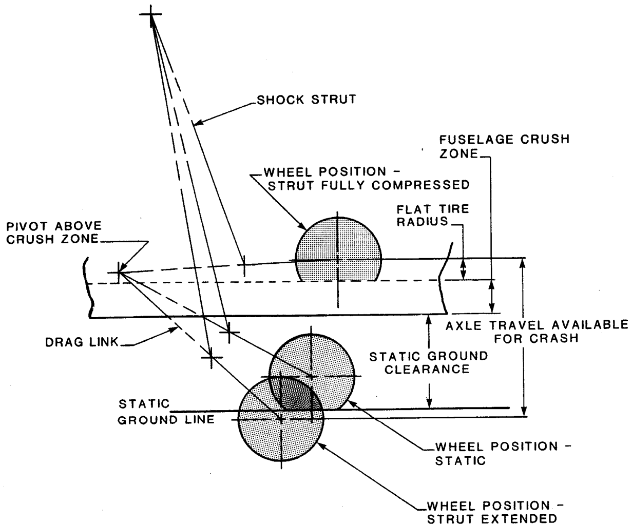
FIGURE 72. GEAR GEOMETRY SELECTED TO CONTINUE ABSORBING ENERGY DURING CRUSHING OF FUSELAGE FLOOR.
