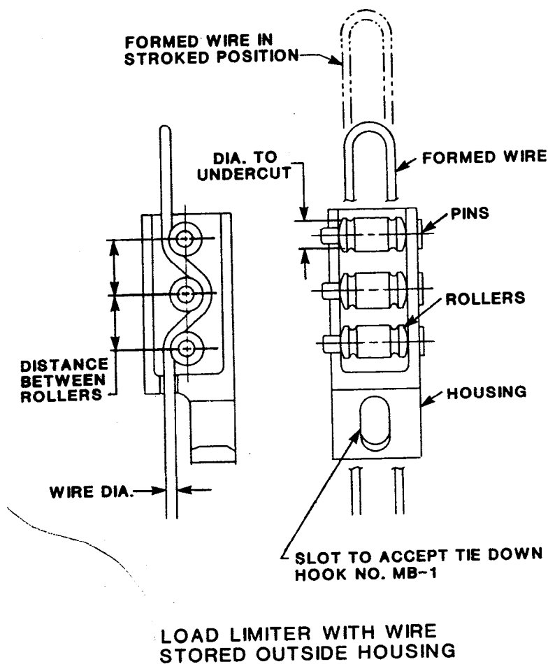
FIGURE 64. CARGO RESTRAINT LOAD LIMITER.
