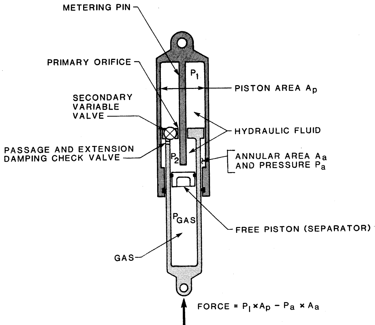
FIGURE 75. AIR/OIL OLEO SCHEMATIC.
