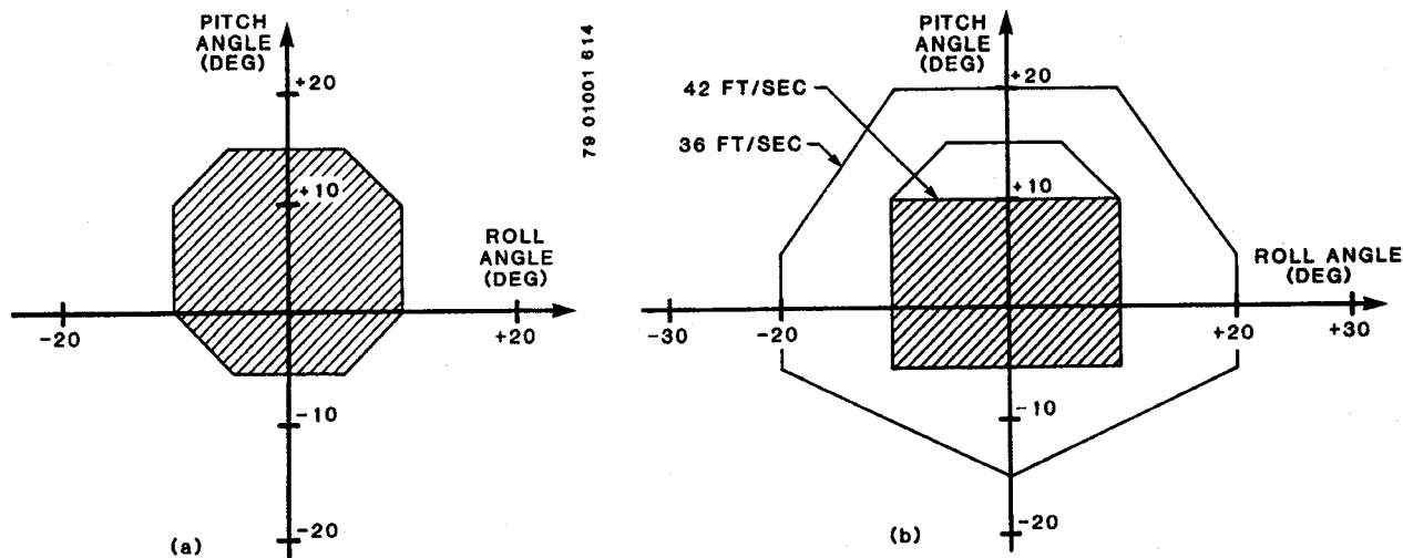
FIGURE 37. ROLL AND PITCH ATTITUDE ENVELOPES.
