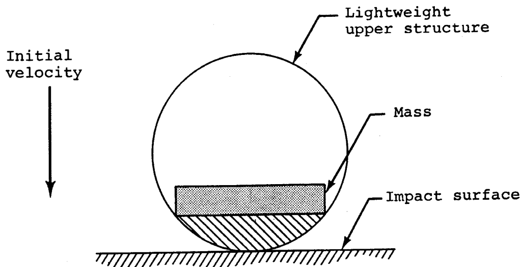
FIGURE 35. FUSELAGE STRUCTURE WITHOUT OVERHEAD MASS ITEMS (IDEALIZATION).
