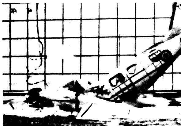
4. COCKPIT LIVABLE VOLUME TOTALLY COLLAPSED
