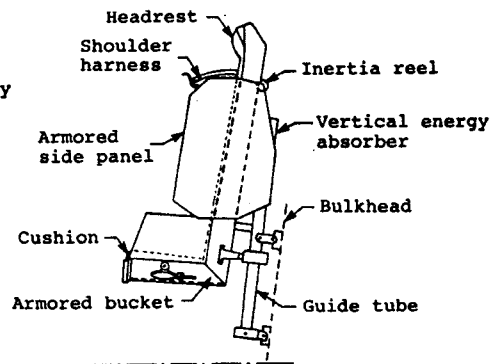
(b) Crewseat, armored bucket, bulkhead-mounted
