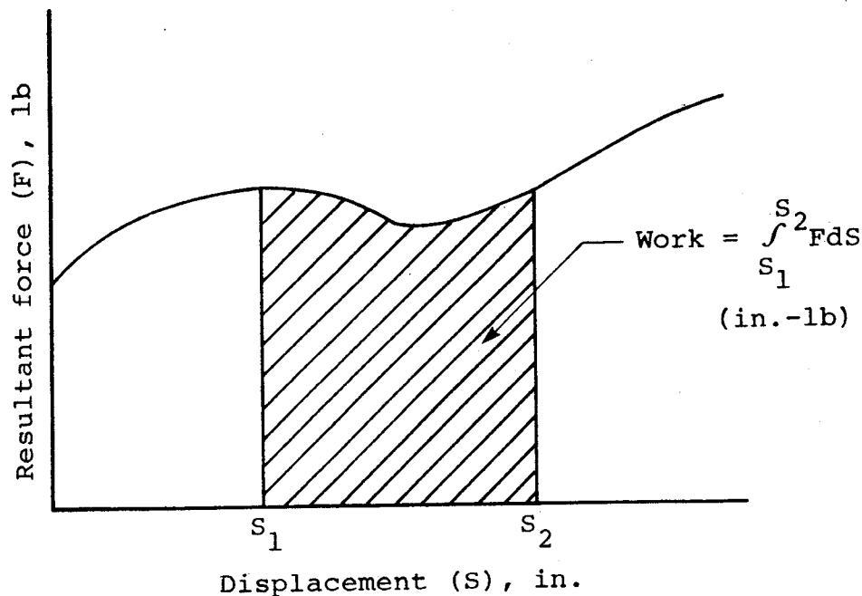
FIGURE 82. DEFINITION OF WORK.
