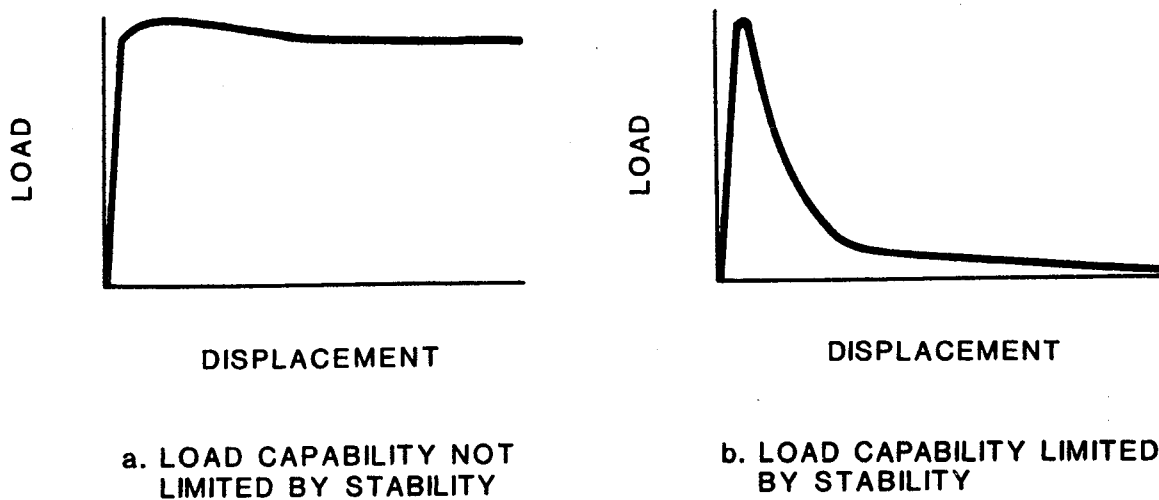
FIGURE 97. TYPICAL LOAD-DISPLACEMENT CHARACTERISTICS FOR AIRFRAME STRUCTURE.
