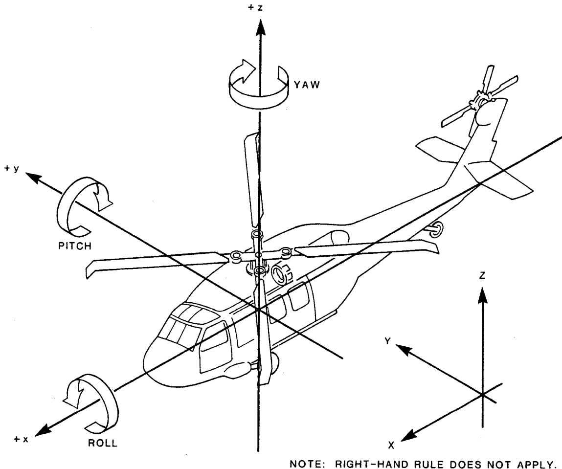
FIGURE 3. AIRCRAFT COORDINATES AND ATTITUDE DIRECTIONS.
