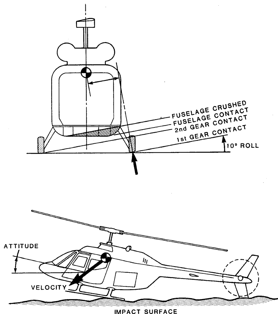
FIGURE 25. DIRECTION AND ATTITUDE OF IMPACT.
