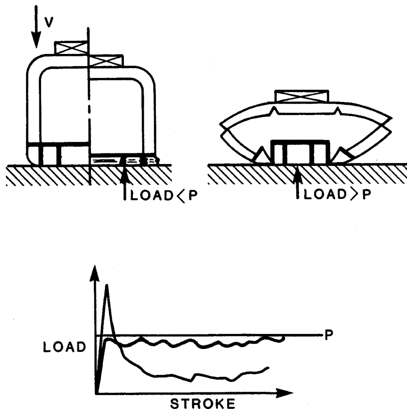
FIGURE 36. VERTICAL IMPACT CRUSHING LOADS.
