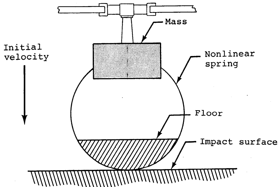
FIGURE 33. FUSELAGE STRUCTURE WITH OVERHEAD LARGE MASS ITEMS (IDEALIZATION).
