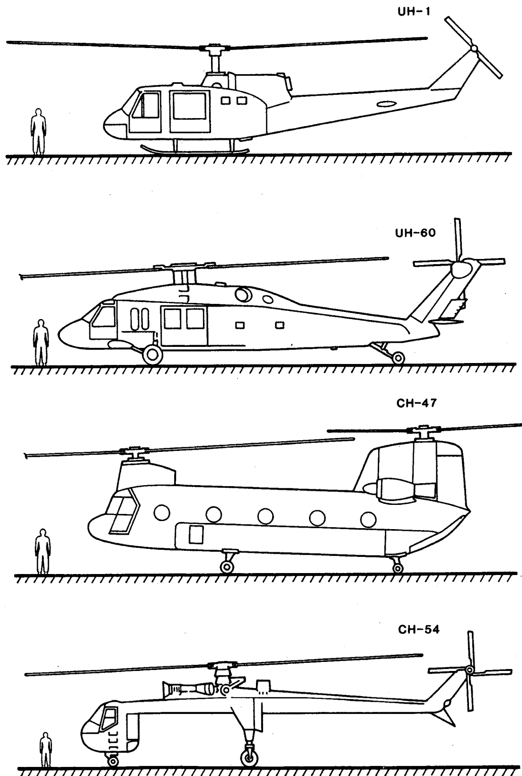
FIGURE 11. SIDE ELEVATIONS OF TYPICAL U.S. ARMY UTILITY AND CARGO HELICOPTERS.
