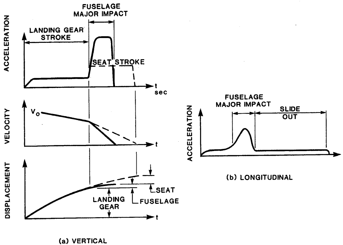
FIGURE 32. TYPICAL VERTICAL AND LONGITUDINAL CRASH PULSES.
