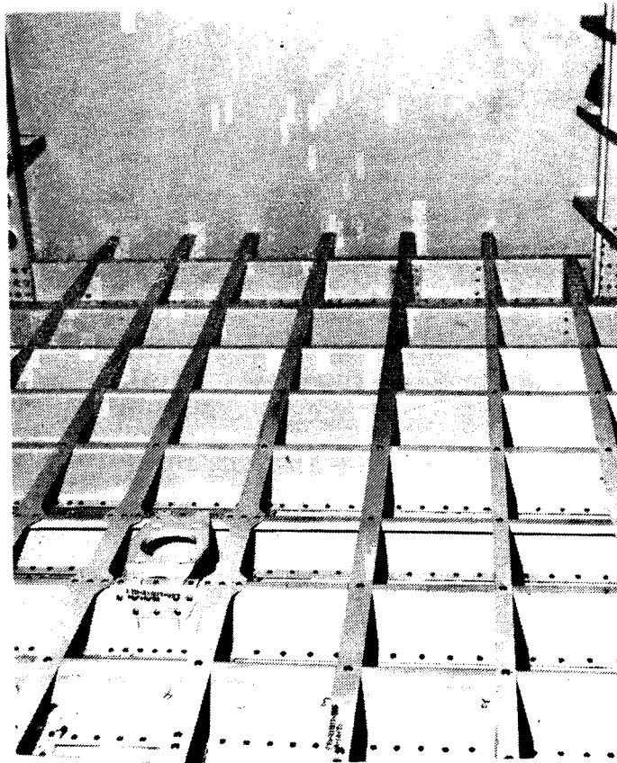
FIGURE 59. TYPICAL INTERIOR SUPPORT STRUCTURE FOR FUEL CELL.
