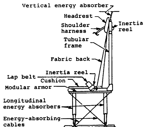
(c) Gunner seat, side-facing frame construction
