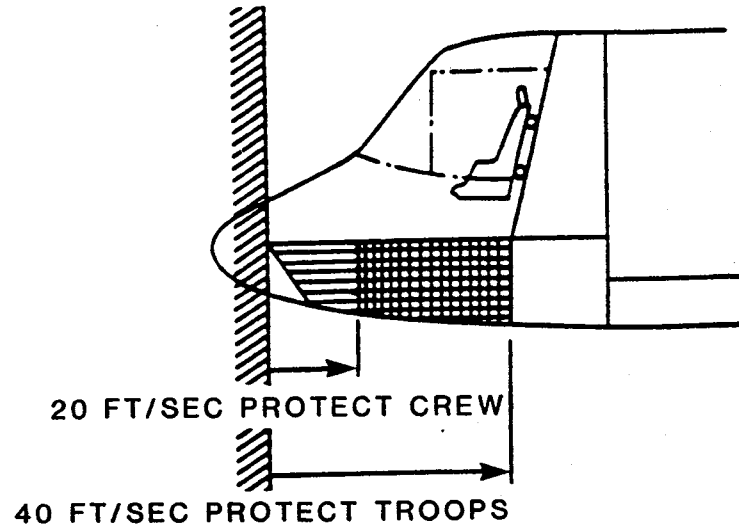
FIGURE 48. LONGITUDINAL IMPACT DESIGN CRITERIA.
