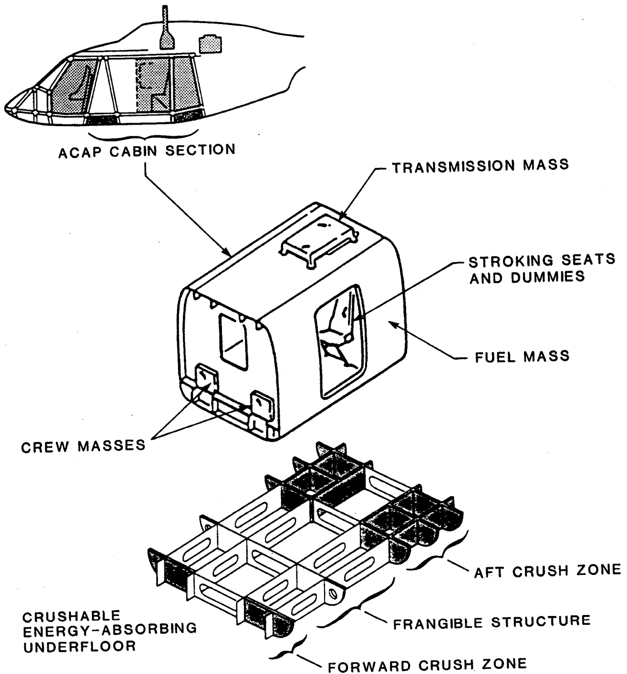
FIGURE 42. COMPOSITE CABIN TEST SECTION.
