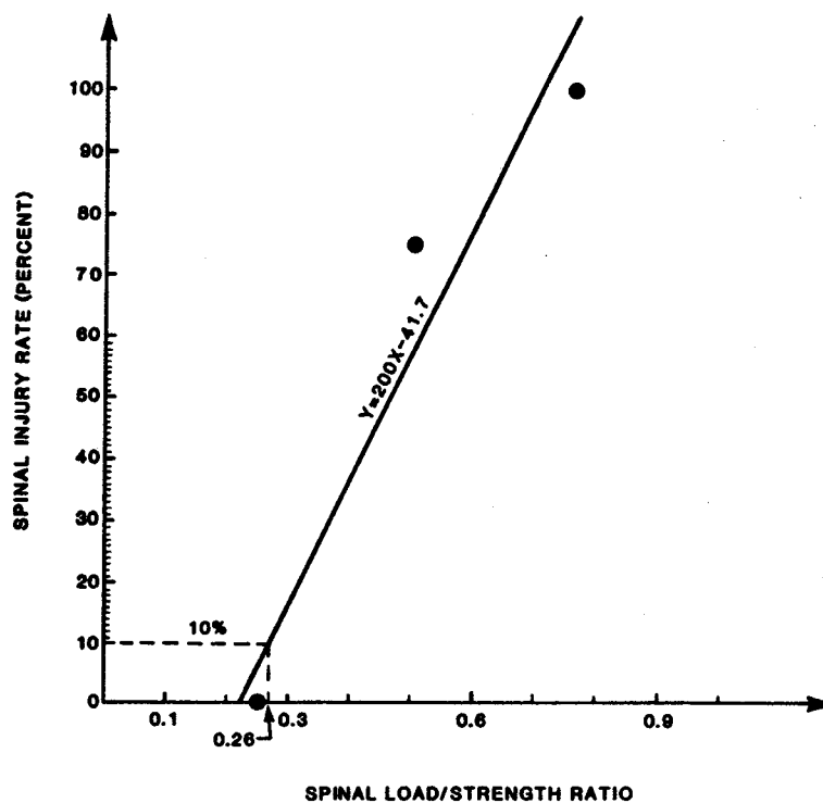
FIGURE 30. SPINAL INJURY RATE AS A FUNCTION OF SPINAL LOAD/STRENGTH RATIO (SLSR). (REFERENCE 41)
