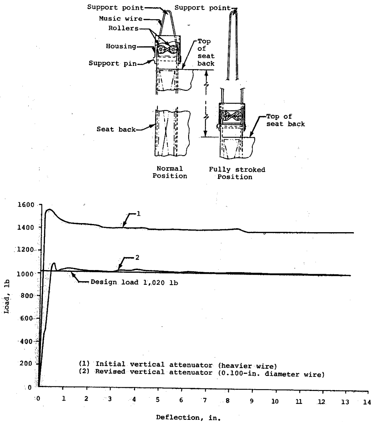
FIGURE 43. TROOP SEAT TENSION ENERGY ABSORBER INCLUDING CHARACTERISTICS FOR TWO WIRE DIAMETERS.
