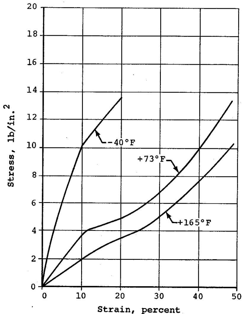
FIGURE 116. STRESS-STRAIN CURVES FOR POLYETHYLENE FOAM. (REFERENCE 154)
