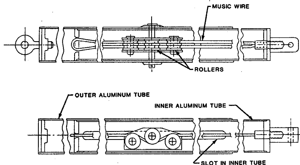
FIGURE 44. TUBULAR STRUT WIRE-BENDING ENERGY ABSORBER. (REFERENCE 35)
