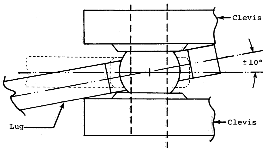
FIGURE 13. UNIVERSAL RELEASE OF A JOINT.
