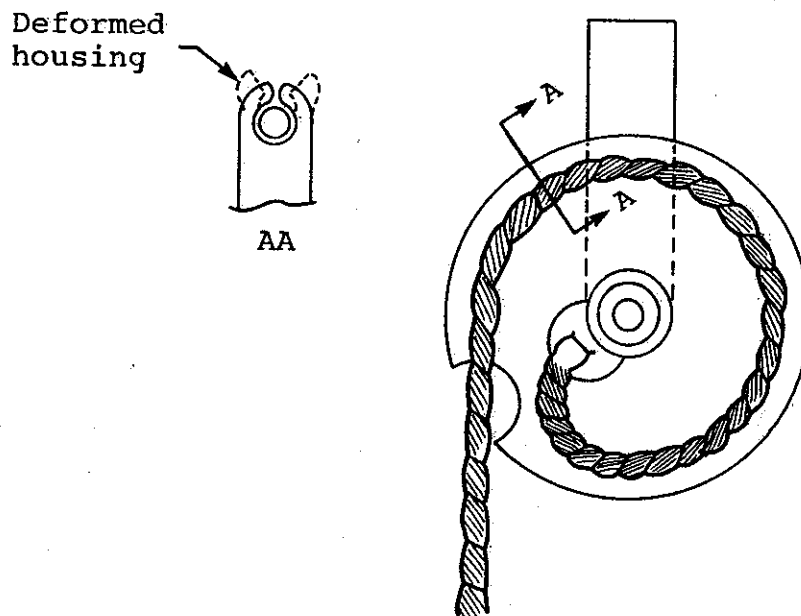
FIGURE 51. TENSION-PULLEY LOAD LIMITER.
