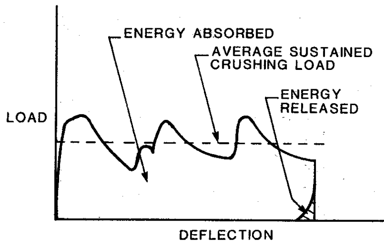
FIGURE 56. TYPICAL LOAD-DEFLECTION CURVE OF ALUMINUM TUBE. (REFERENCE 85)
