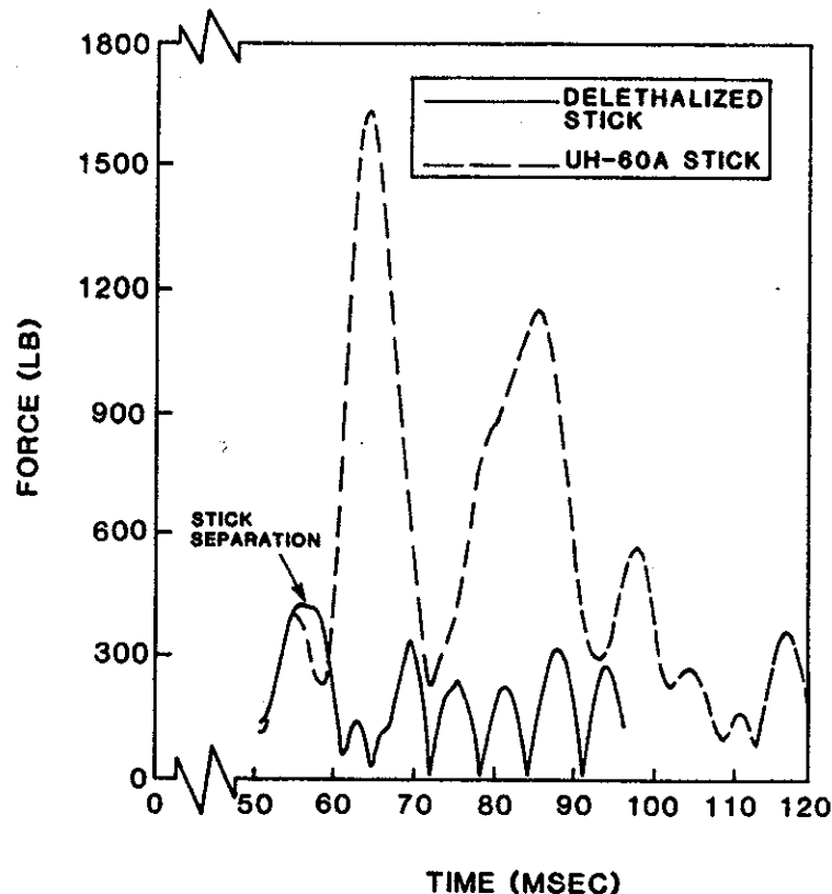
FIGURE 109. STICK LOAD. (REFERENCE 141)
