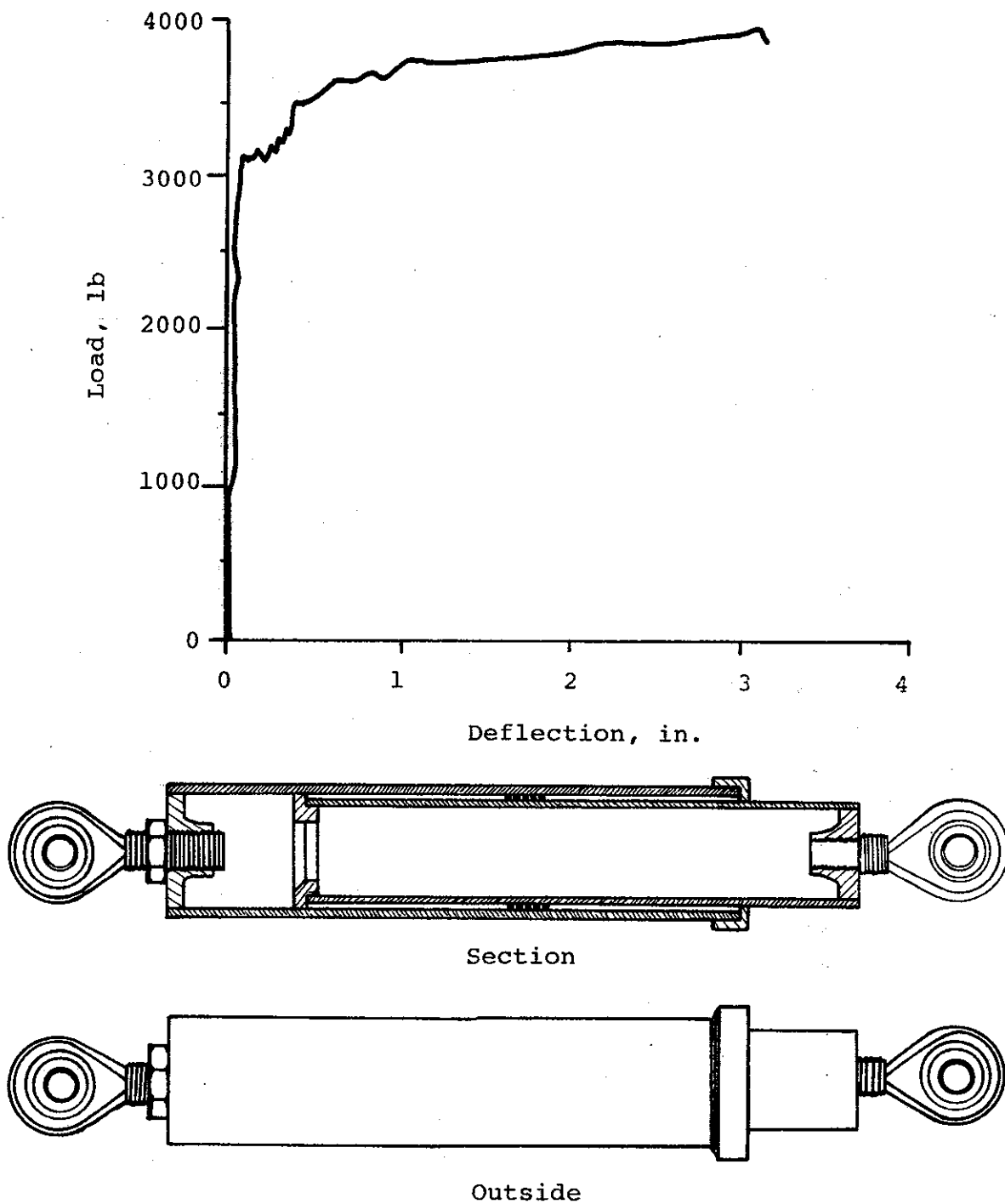
FIGURE 46. ROLLING TORUS ENERGY ABSORBER.
