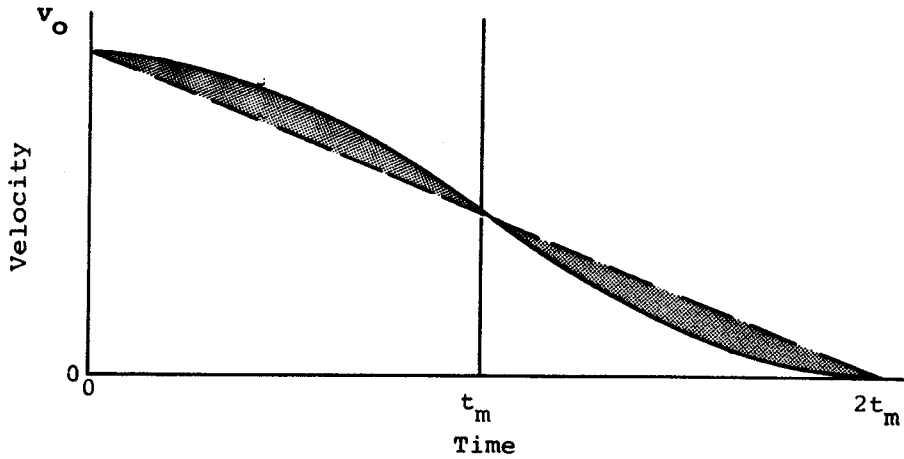
FIGURE 18. AIRFRAME VELOCITY-TIME CURVE.
