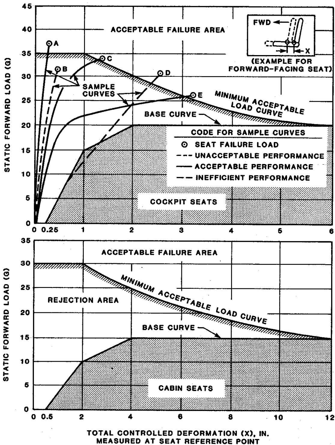
FIGURE 85. SEAT FORWARD LOAD AND DEFLECTION REQUIREMENTS FOR ALL TYPES OF ARMY AIRCRAFT (FORWARD DESIGN PULSE).
