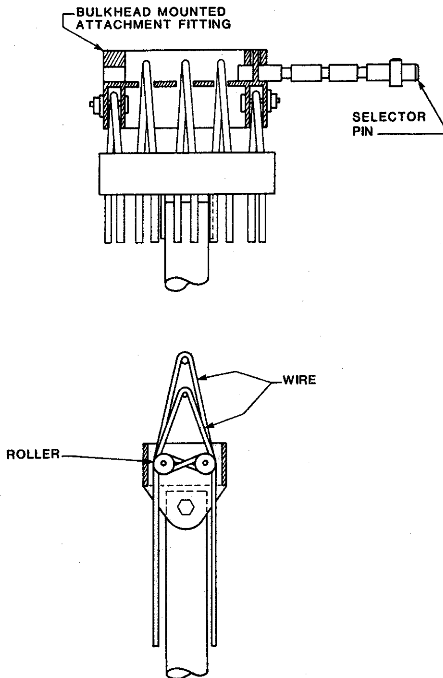
FIGURE 79. MULTILOAD ENERGY ABSORBER.
