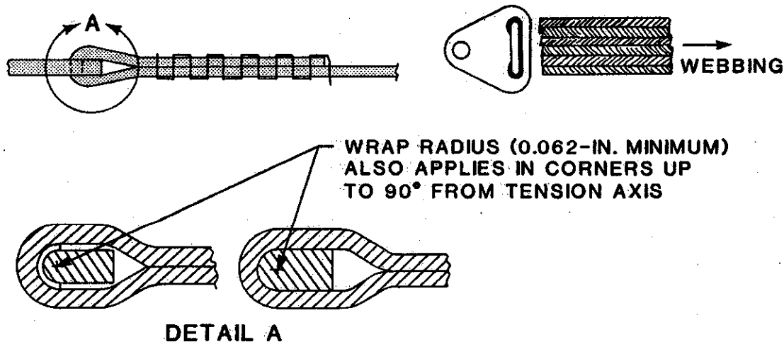
FIGURE 75. WRAP RADIUS FOR WEBBING JOINTS.
