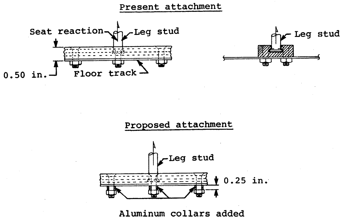
FIGURE 16. SEAT LEG ANCHORAGE TO FLOOR TRACK.
