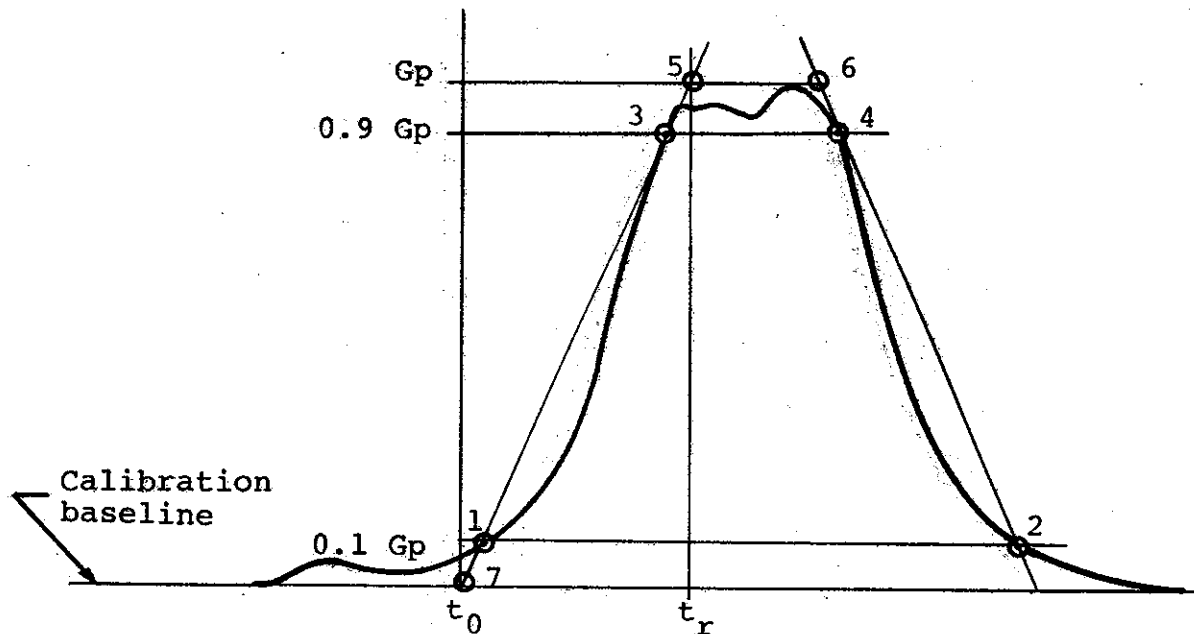
FIGURE 83. GRAPHIC APPROXIMATION EXAMPLE. (REFERENCE 122)
