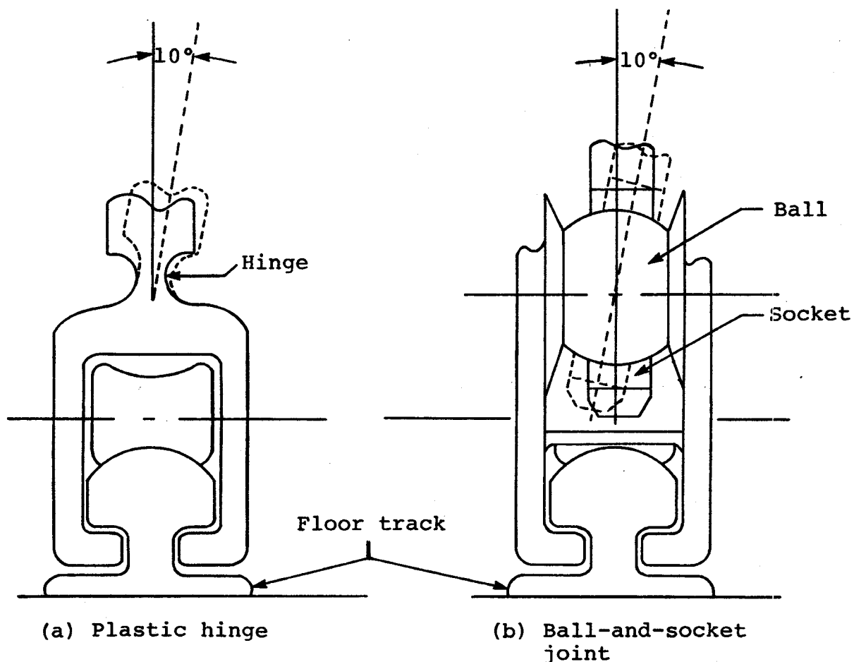
FIGURE 7. CONCEPTS FOR RELEASE OF FLOOR-DISTORTION-INDUCED MOMENTS.
