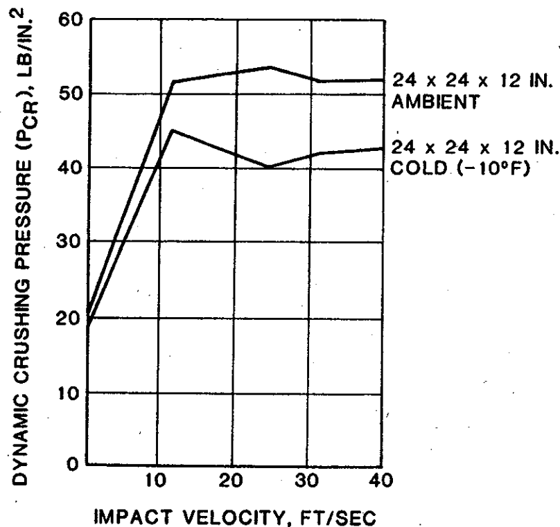
FIGURE 123. DYNAMIC CRUSHING PRESSURE VERSUS IMPACT VELOCITY FOR TESTS AT TWO TEMPERATURES.
