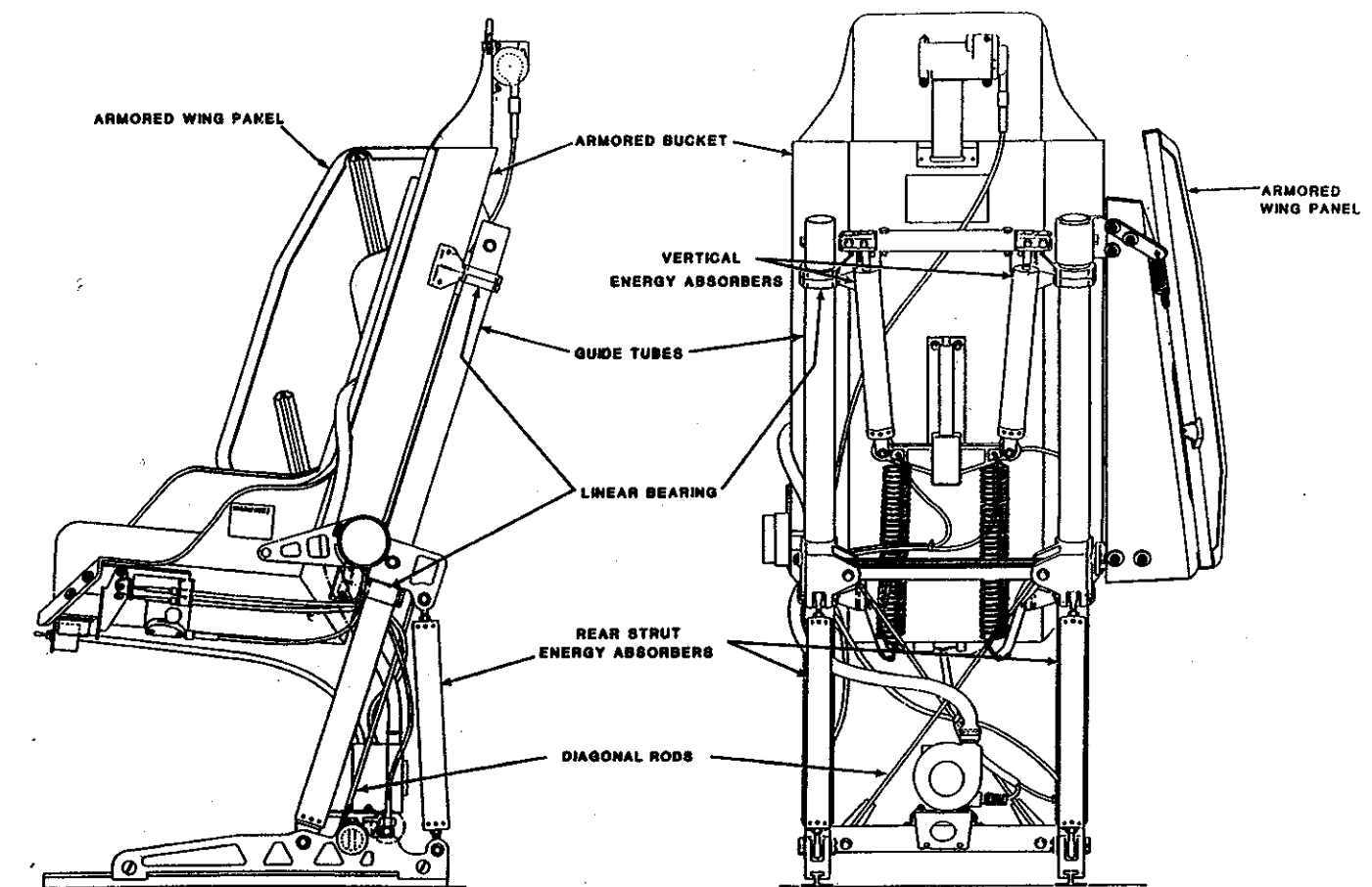
FIGURE 84. CH-53 CREWSEAT.
