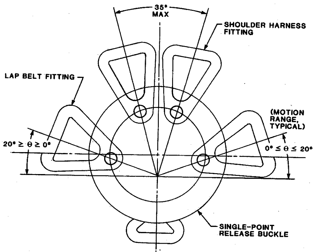
FIGURE 68. BUCKLE FITTING ATTACHMENT AND MOTION ANGLES.
