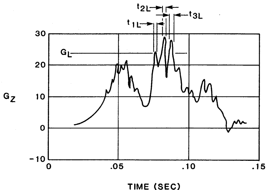
FIGURE 27. TYPICAL G_z VERSUS TIME PLOTS.
