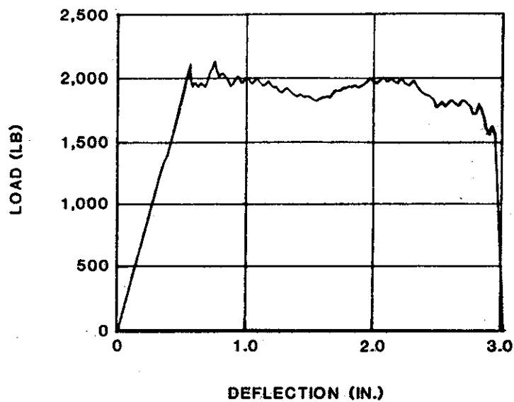
FIGURE 89. LOAD-VERSUS-DEFLECTION CURVE, ENERGY ABSORBER INERTIA REEL. (REFERENCE 125)
