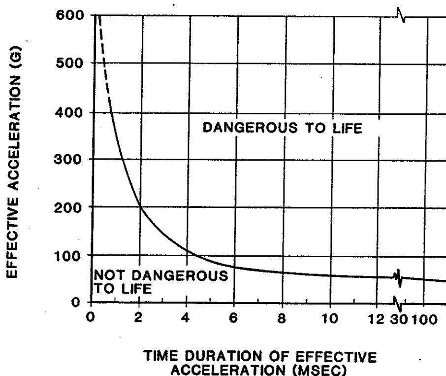
FIGURE 103. WAYNE STATE TOLERANCE CURVE FOR THE HUMAN BRAIN IN FOREHEAD IMPACTS AGAINST PLANE, UNYIELDING SURFACES. (REFERENCE 132)
