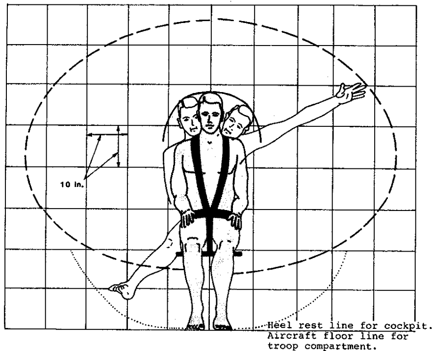
FIGURE 96. FULL-RESTRAINT EXTREMITY STRIKE ENVELOPE - FRONT VIEW.
