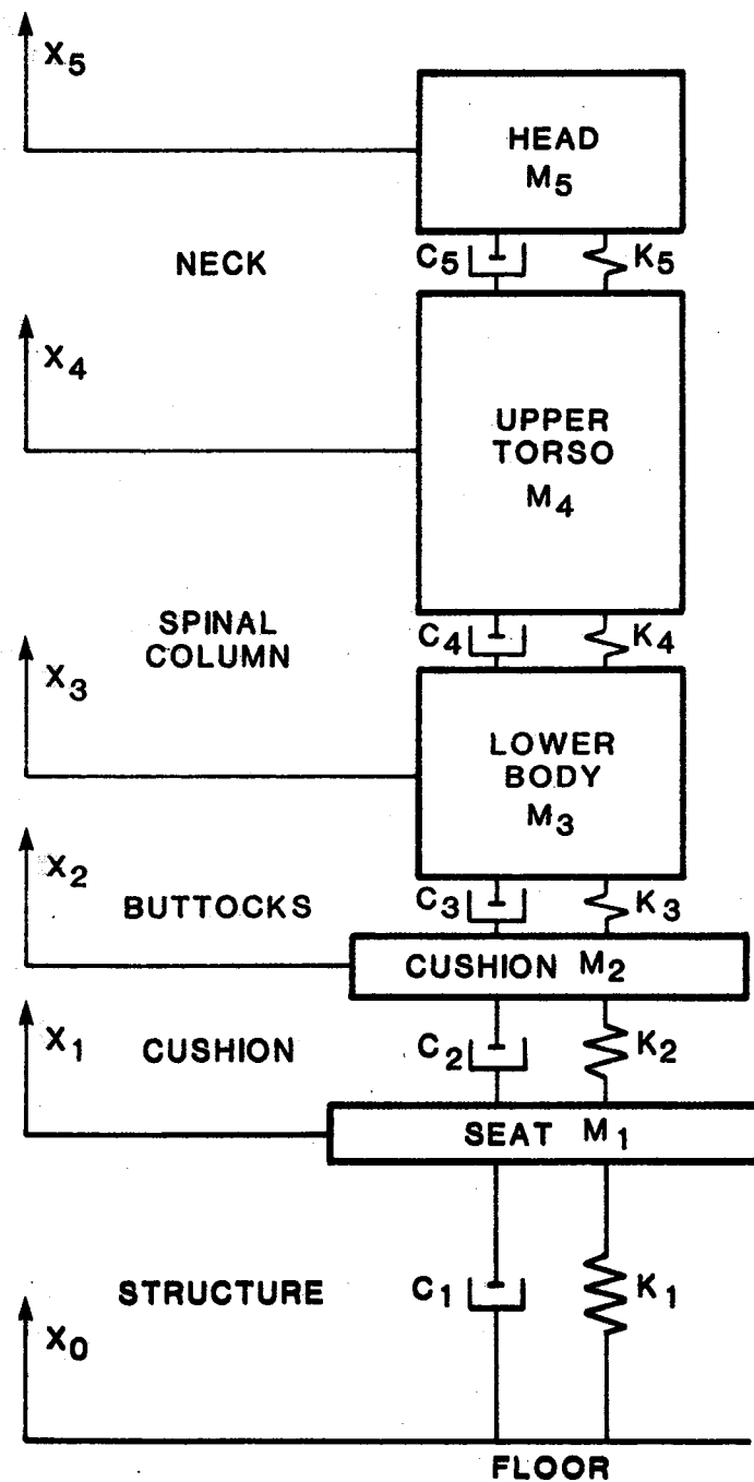
FIGURE 41. LUMPED-PARAMETER MODEL OF SEAT, SEAT CUSHION, AND OCCUPANT.
