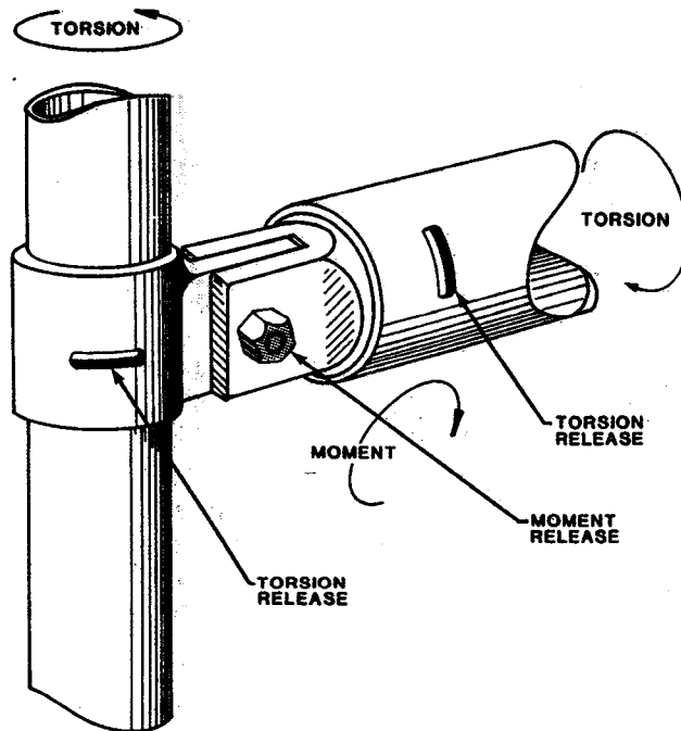
FIGURE 11. FULLY RELEASED JOINT.
