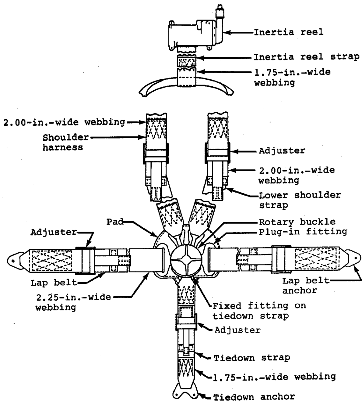
FIGURE 77. AIRCREW RESTRAINT SYSTEM.
