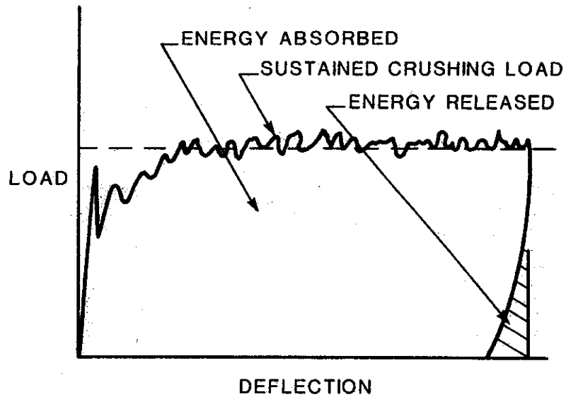
FIGURE 55. TYPICAL LOAD-DEFLECTION CURVE OF COMPOSITE TUBE. (REFERENCE 85)
