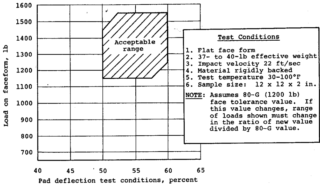
FIGURE 119. LOAD-DISTRIBUTING MATERIAL EVALUATION CRITERIA. (REFERENCE 156)
