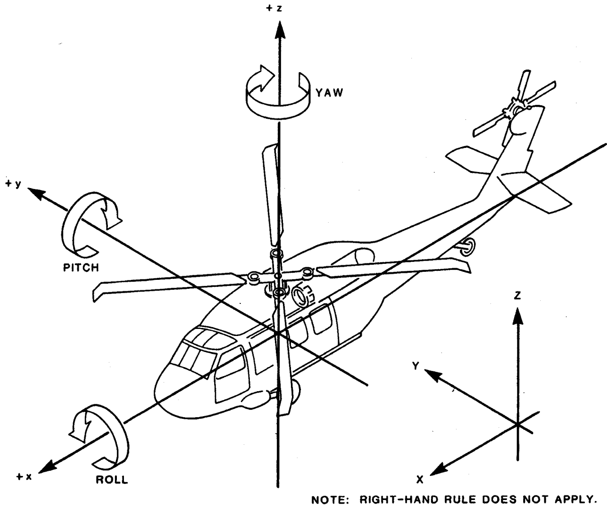
FIGURE 1. AIRCRAFT COORDINATES AND ATTITUDE DIRECTIONS.
