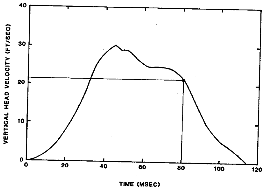
FIGURE 106. HEAD VELOCITY - VERTICAL COMPONENT. (REFERENCE 133)
