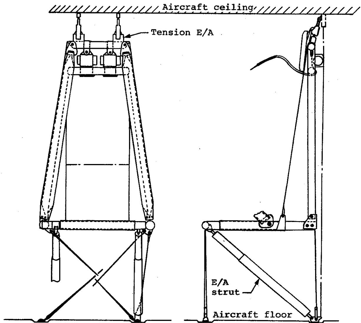
FIGURE 42. CRASH-RESISTANT TROOP SEAT. (REFERENCE 75)
