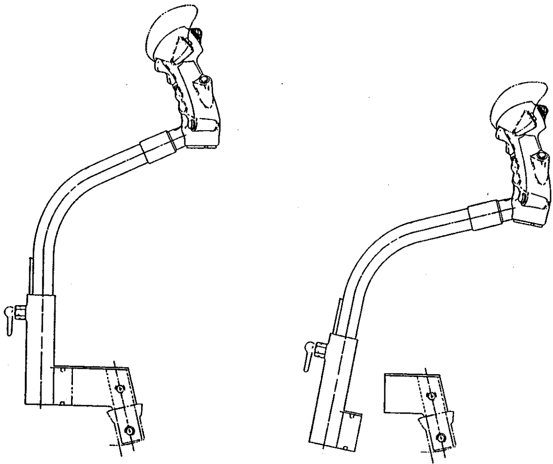
FIGURE 108. DELETHALIZED CYCLIC CONTROL STICK. (REFERENCE 132)
