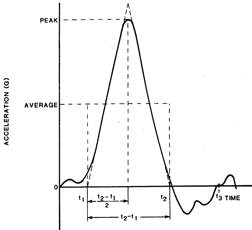
FIGURE 2. TYPICAL AIRCRAFT FLOOR ACCELERATION PULSE.
