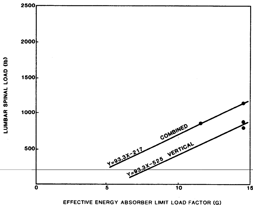
FIGURE 29. CORRELATION BETWEEN PEAK LUMBAR SPINAL LOAD MEASURED IN THE INSTRUMENTED ANTHROPOMORPHIC DUMMY AND ENERGY ABSORBER LIMIT-LOAD FACTOR. (REFERENCE 41)
