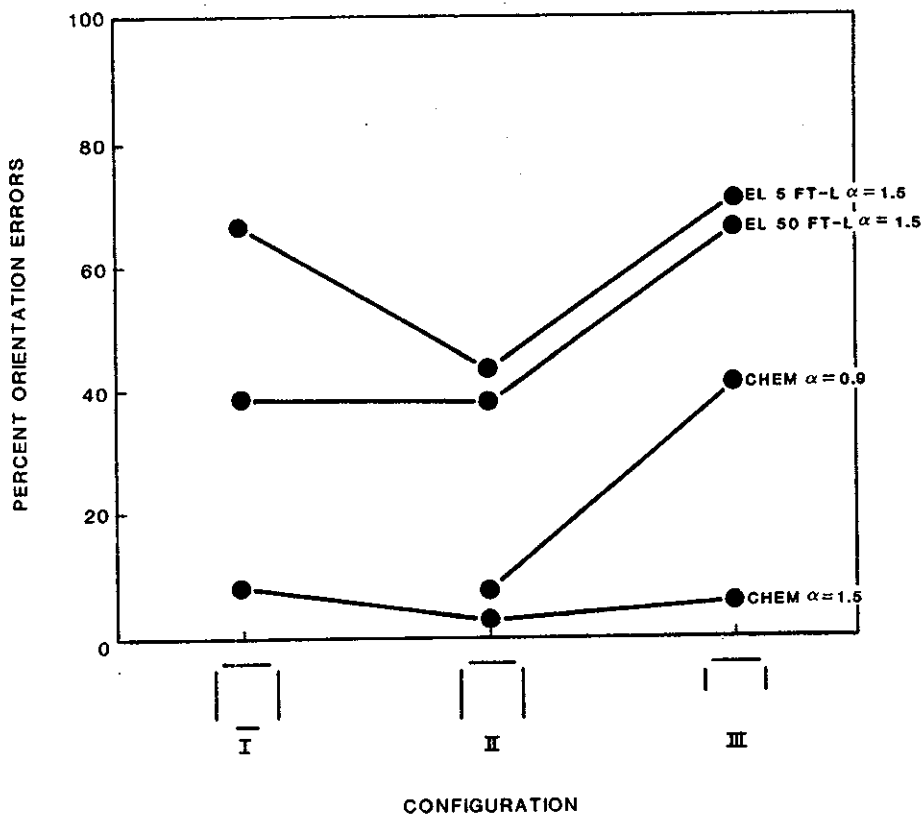
FIGURE 76. PERCENTAGE OF TRIALS ON WHICH THE SUBJECTS COULD NOT CORRECTLY IDENTIFY THE ORIENTATION OF THE THREE LIGHTING CONFIGURATIONS FOR VARIOUS LIGHTS OVER THE THREE DISTANCES IN WATER OF TWO TURBIDITIES. THE CHEMICAL LIGHTS WERE NOT TESTED IN CONFIGURATION I AT A TURBIDITY OF \alpha \approx 0.9 .
