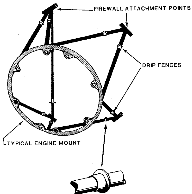
FIGURE 51. FUEL FLOW DIVERTERS.
