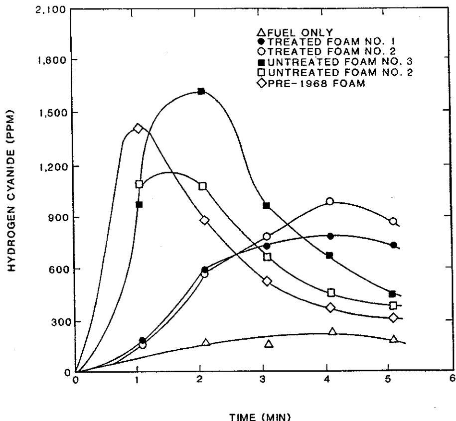
FIGURE 61. HYDROGEN CYANIDE CONCENTRATIONS FROM BURN TESTS OF COATED AND UNCOATED POLYURETHANE FOAMS.
