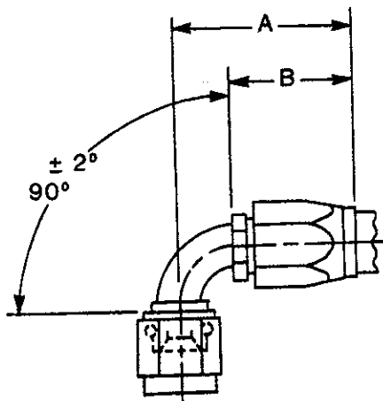
FIGURE 25. STANDARD HOSE FITTING DIMENSIONS.
