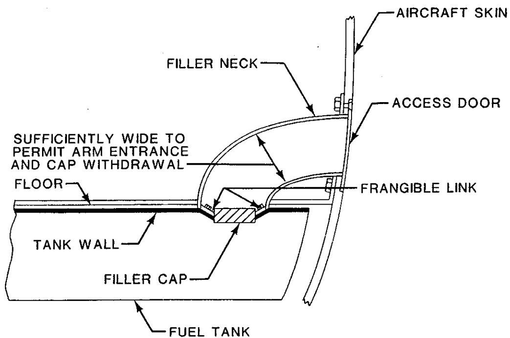
FIGURE 34. FRANGIBLE FILLER NECK INSTALLATION.
