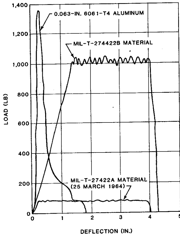
FIGURE 15. RESISTANCE OF MATERIALS TO TEARING.
