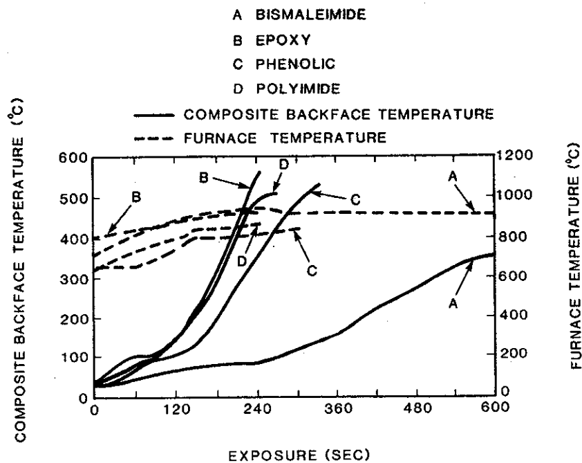
FIGURE 65. THERMAL EFFICIENCY OF EXPERIMENTAL PANELS WITH VARIOUS FACE SHEET MATERIALS.
