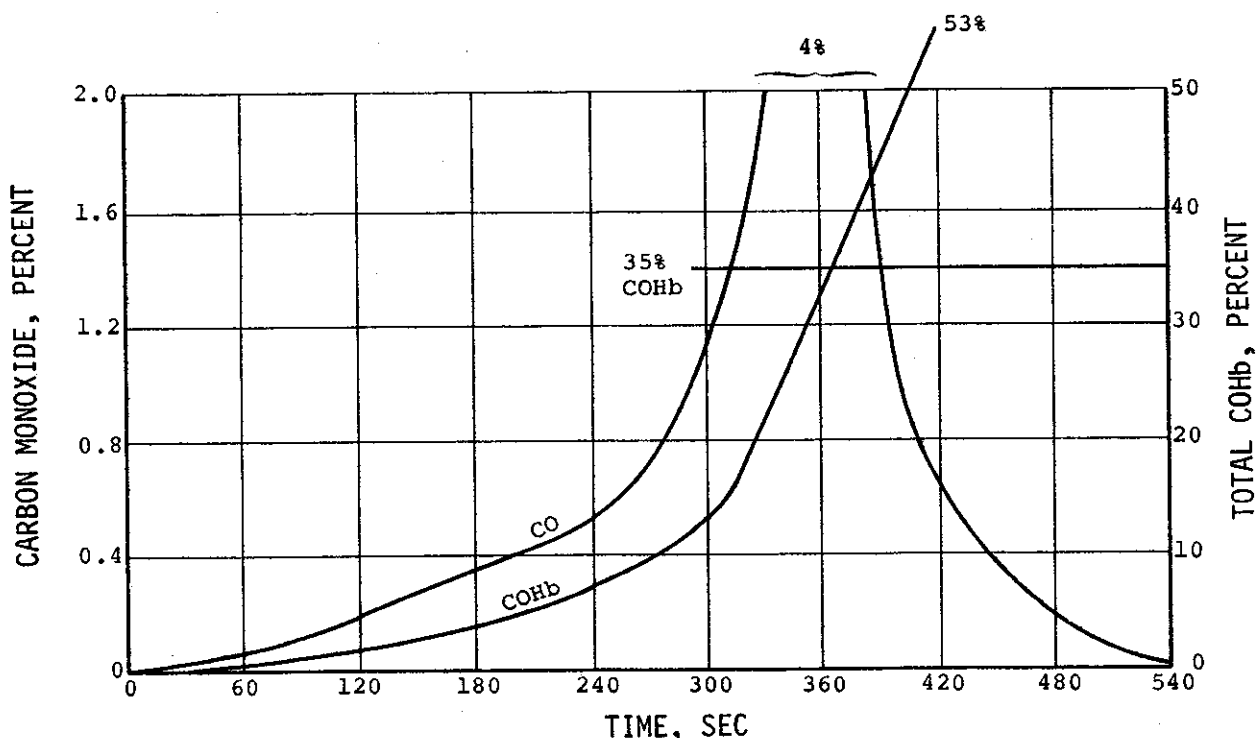
FIGURE 6. AVERAGE RECORDED CO CONCENTRATIONS AND CALCULATED COHb LEVELS IN LARGE, CRASHED, BURNING, PASSENGER/CARGO-CARRYING FIXED-WING AIRCRAFT.
