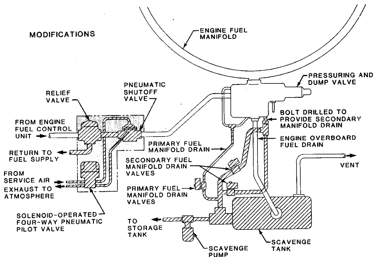
FIGURE 47. SCHEMATIC DIAGRAM SHOWING FUEL SHUTOFF AND DRAIN SYSTEM IN J57 ENGINE CRASH-FIRE PROTECTION SYSTEM.
