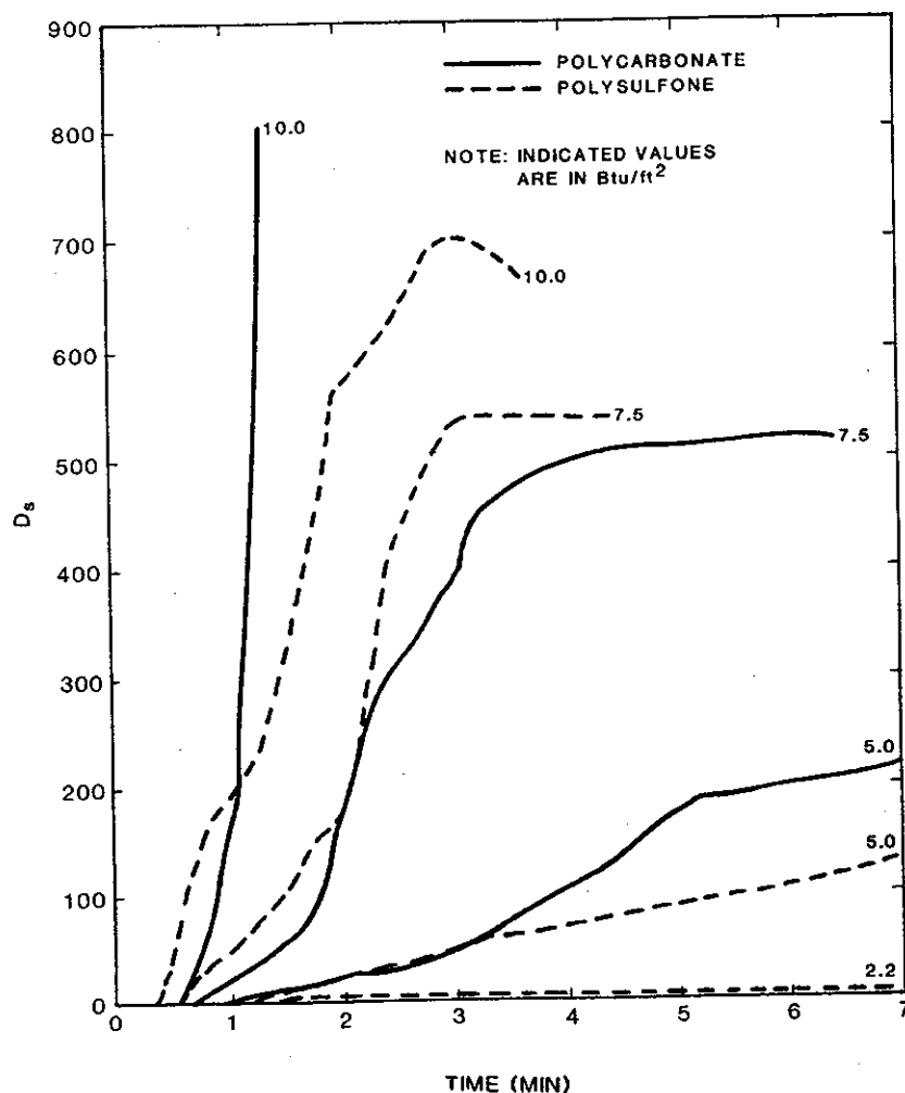
FIGURE 56. SMOKE PRODUCTION VERSUS HEAT FLUX - POLYCARBONATE AND POLYSULFONE SHEETS.
