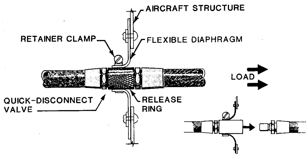
FIGURE 23. MODIFIED QUICK-DISCONNECT LINE-TO-LINE VALVE. (PULL OF DESIGNATED HOSE WILL CAUSE VALVE SEPARATION.)
