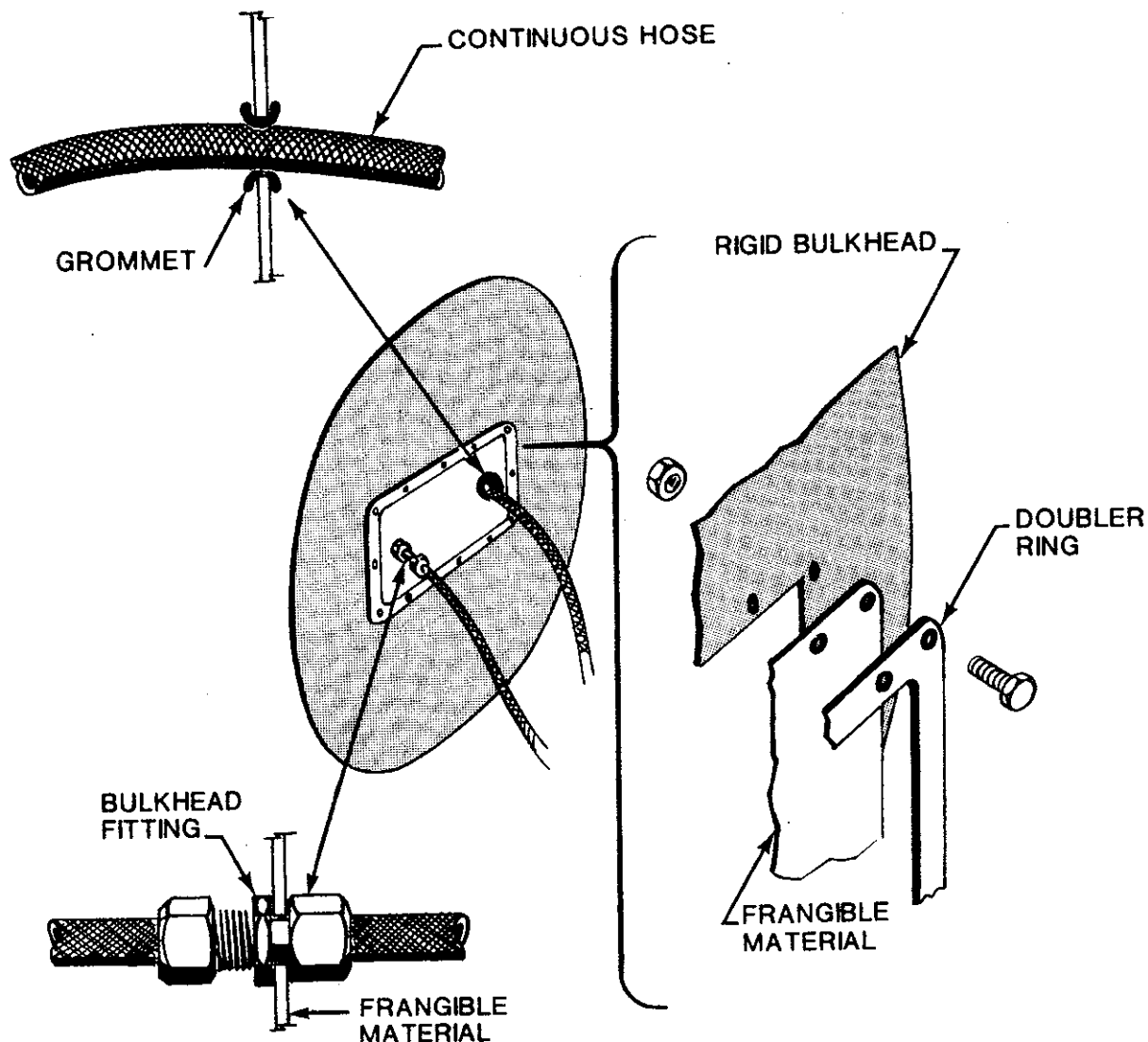
FIGURE 27. HOSE STABILIZING WITH FRANGIBLE STRUCTURE.
