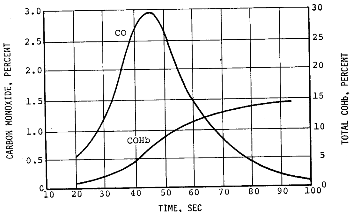
FIGURE 7. AVERAGE RECORDED CO CONCENTRATIONS AND CALCULATED COHb LEVELS IN LARGE, CRASHED, BURNING, PASSENGER/CARGO-CARRYING HELICOPTERS.
