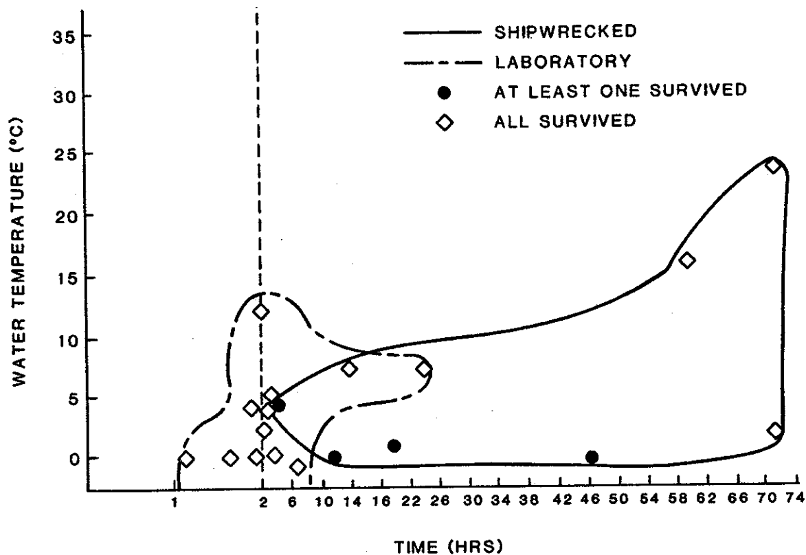
FIGURE 79. TOLERANCE TIME FOR DIFFERENT WATER TEMPERATURES WHILE IN LIFE RAFTS.
