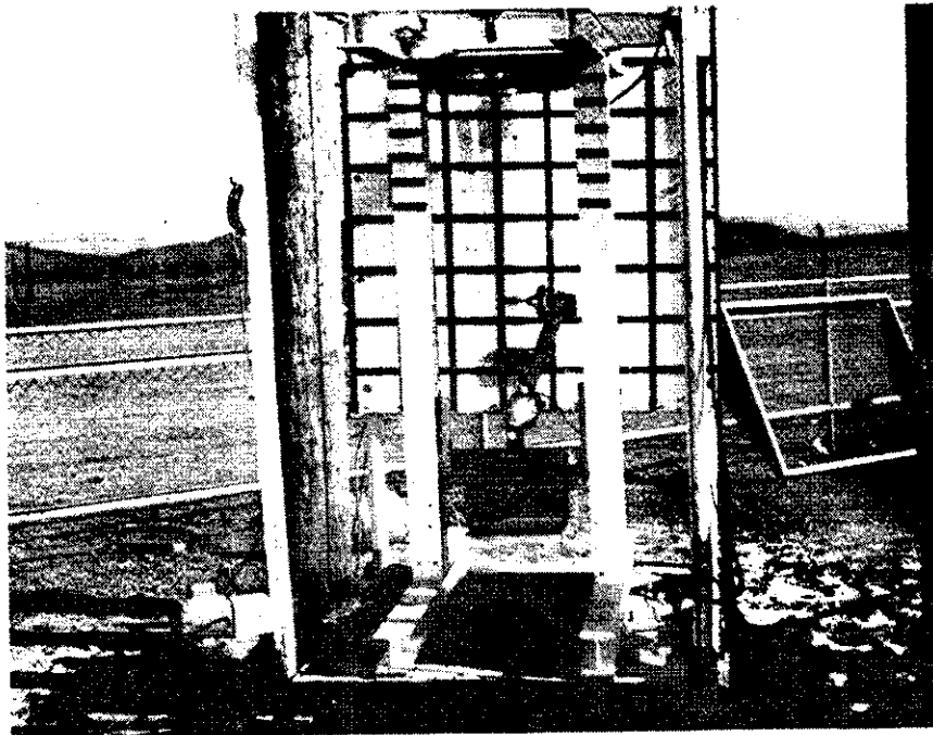
FIGURE 19. TYPICAL FUEL TANK FITTING PULLOUT FOLLOWING DYNAMIC TEST.
