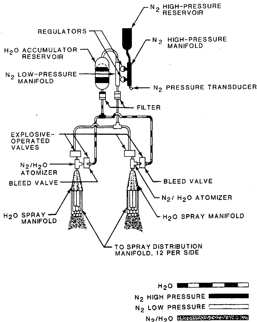
FIGURE 45. HOT SURFACE INERTING SYSTEM.
