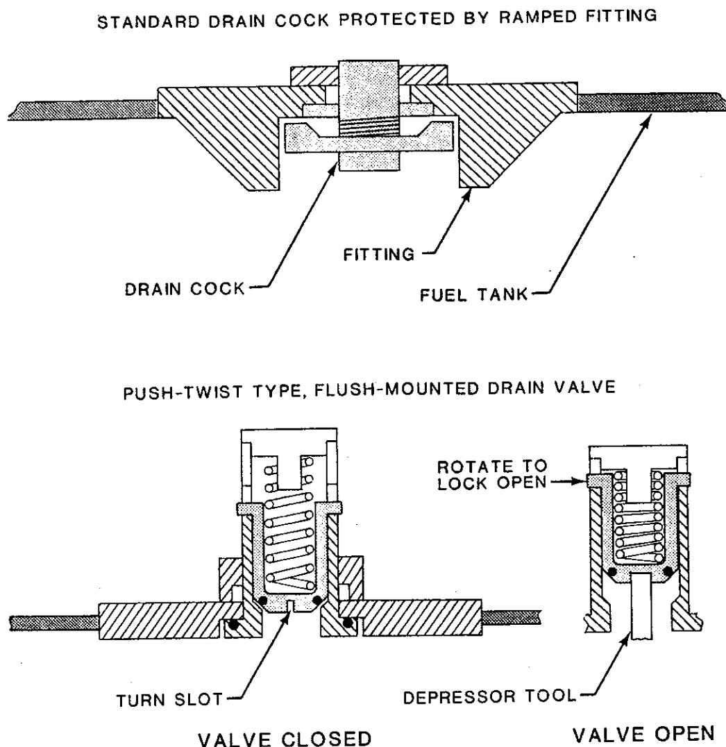
FIGURE 38. DESIGN CONCEPTS FOR CRASH-RESISTANT FUEL DRAIN COCKS.
