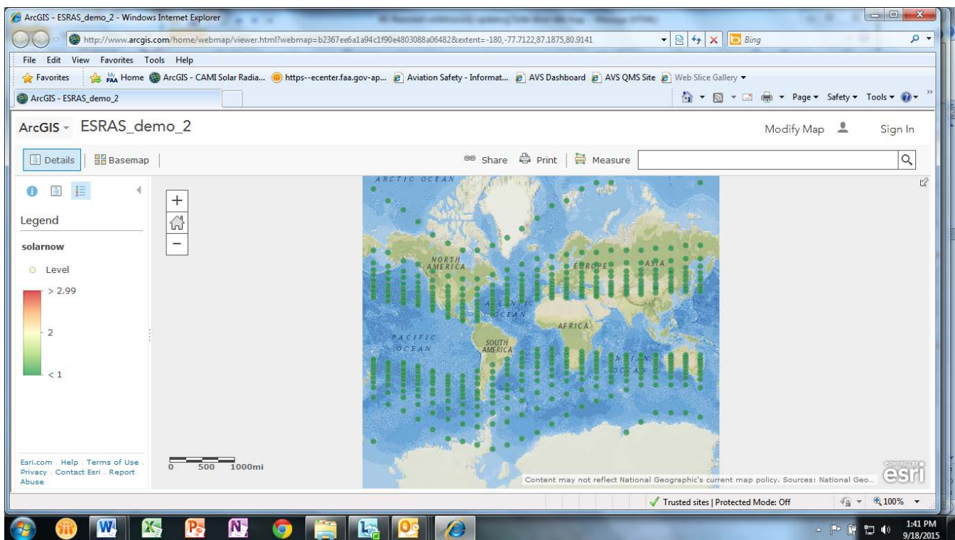
Figure 1. Solar radiation map for normal conditions. Red dots would indicate D_{700} = 3 or more, yellow would indicate D_{700} = 2 , while green indicates D_{700} < 2 .
