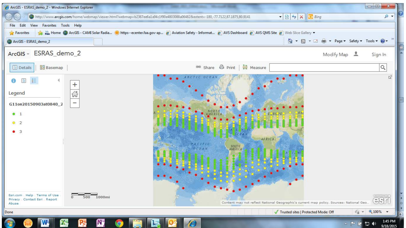
Figure 2. Solar radiation map mockup for conditions during a large solar proton event. Red dots indicate D_{700} = 3 or more, yellow indicates D_{700} = 2 , and green indicates D_{700} < 2 .
