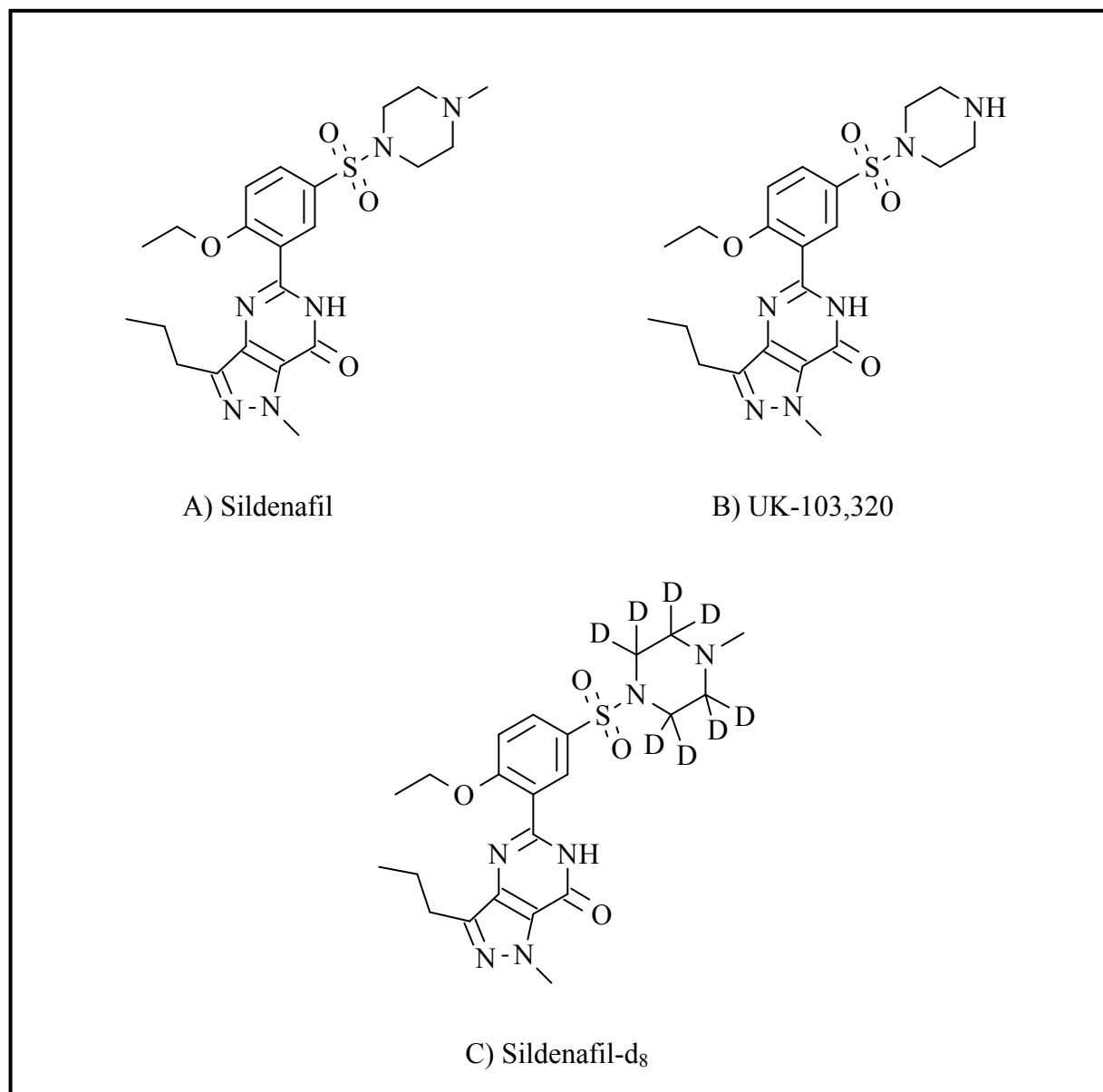
Figure 1. Chemical structures of sildenafil (a), UK-103,320 (b) and sildenafil-d 8 (c).
