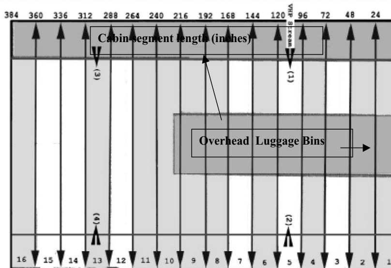
Figure 1. Diagram of the 747 AERF cabin section used to evaluate cabin airflow and VHP distribution. VHP vapor introduction points are identified in sections 5 and 13.
