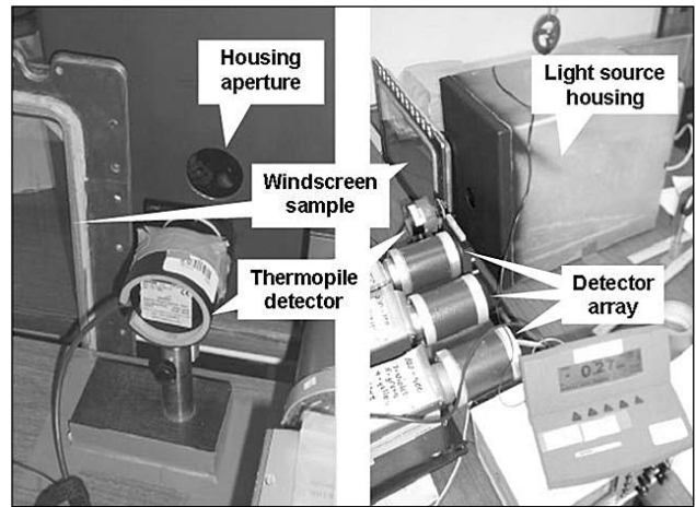
Figure 3. Detector and light source configuration.
