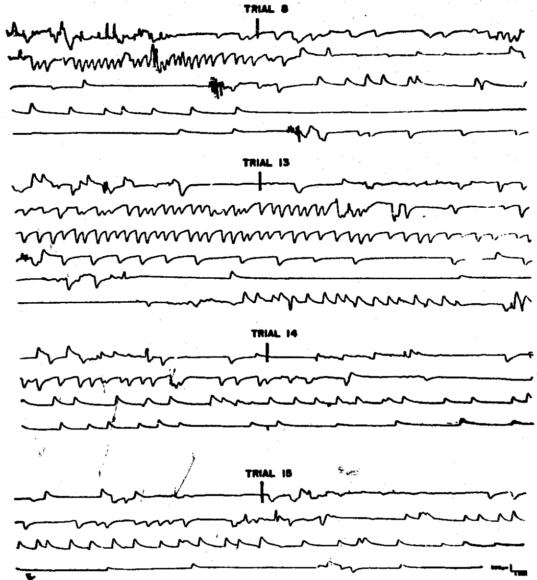
FIGURE 5. Recordings obtained from Cat W. The last 15 seconds of the 30-sec stimulus (applied in total darkness) are depicted. The secondary is brisk on all trials. Note the clear inverted primary nystagmus on Trial 14.
