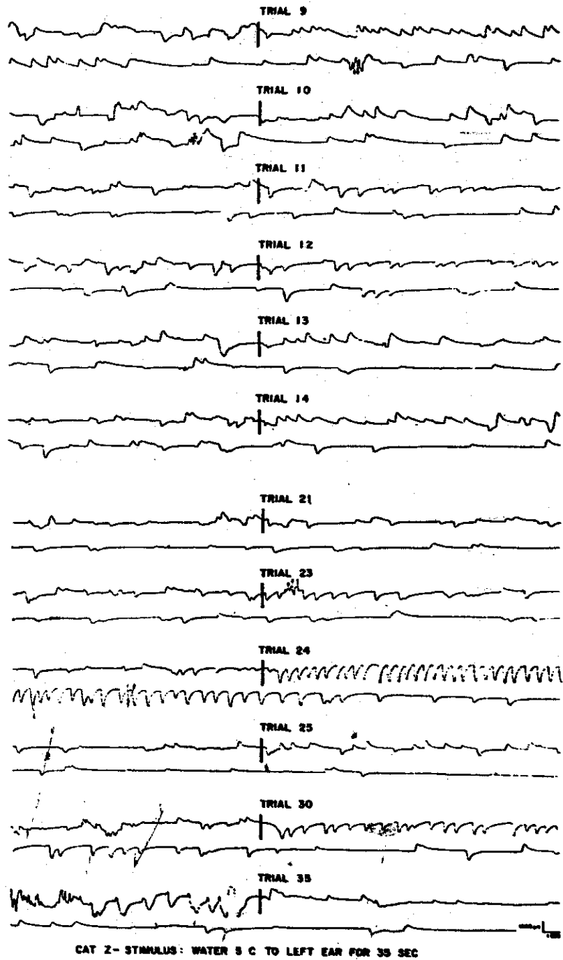
FIGURE 3. Nystagmic responses obtained from left-ear stimulation of Cat Z. The last 15 seconds of the 35-sec stimulus (applied in illumination) are depicted. Vertical bars indicate moment of stimulus-termination and onset of total darkness. Appropriate responses were obtained during the first 10 trials (fast-phase right). Note the particularly vigorous inverted primary responses on Trials 24 and 30.
