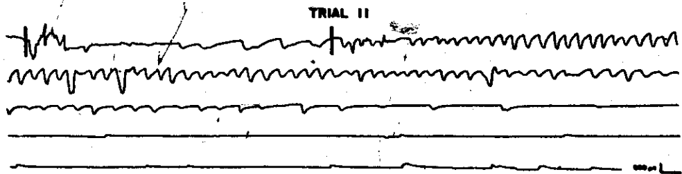
FIGURE 6. Re-test of Cat W one month later with a more potent stimulus. The entire stimulus period (total darkness) is presented. Secondary reactions are clearly evident but no inverted primary responses appeared.
