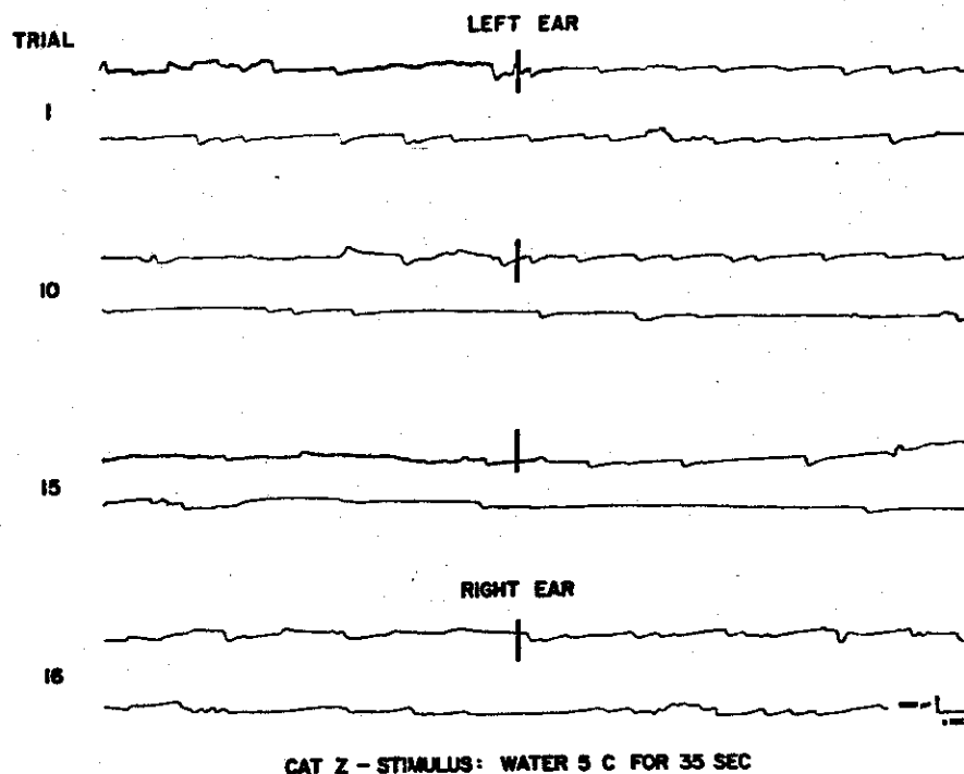
FIGURE 4. Re-test of Cat Z one day later. Test conditions and record markings are the same as in Figure 3. Inverted primary nystagmus appeared during each of the first 15 left-ear trials. The right ear was then stimulated and an appropriate response was elicited (fast-phase left).
