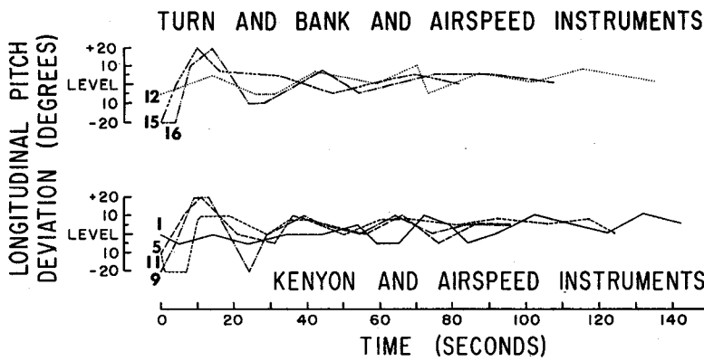
Fig. 5. Pitch control comparisons with Kenyon and T and B instrument.
