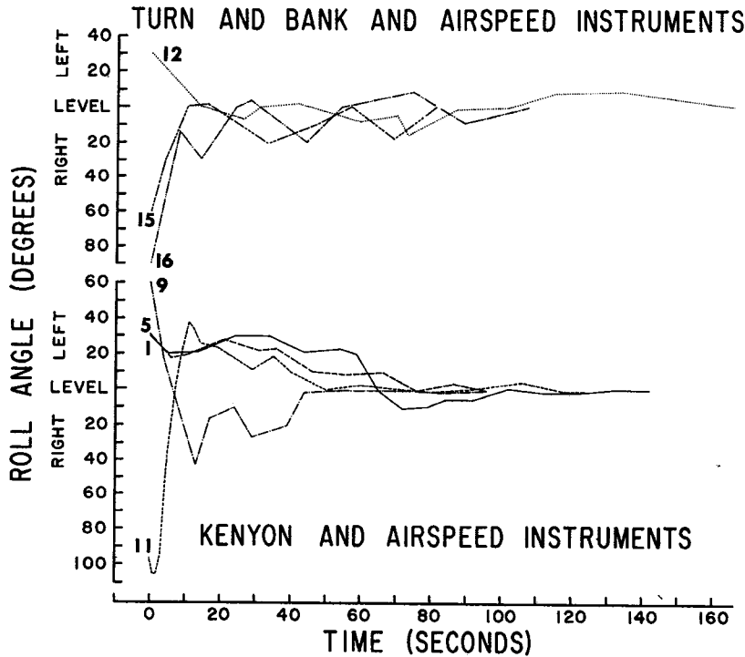
Fig. 3. Comparison of recoveries to straight and level flight between Kenyon and conventional turn and bank instrument.
