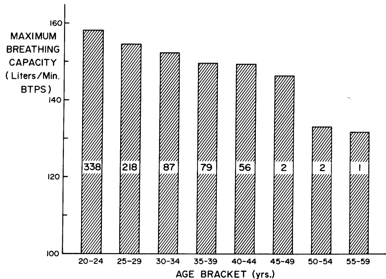
FIGURE 6. Each bar height represents the average maximum breathing capacity (in liters/min.—BTPS) of the individuals within the specified age bracket. The figure within each bar is the number of individuals represented by that bar. These data represent a total of 783 individuals.
