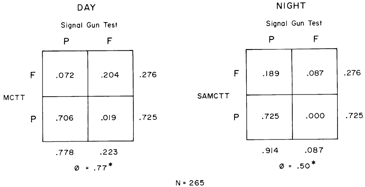
FIGURE 9. Contingency tables and phi coefficients for the signal light gun test and the Color Threshold Tester.
