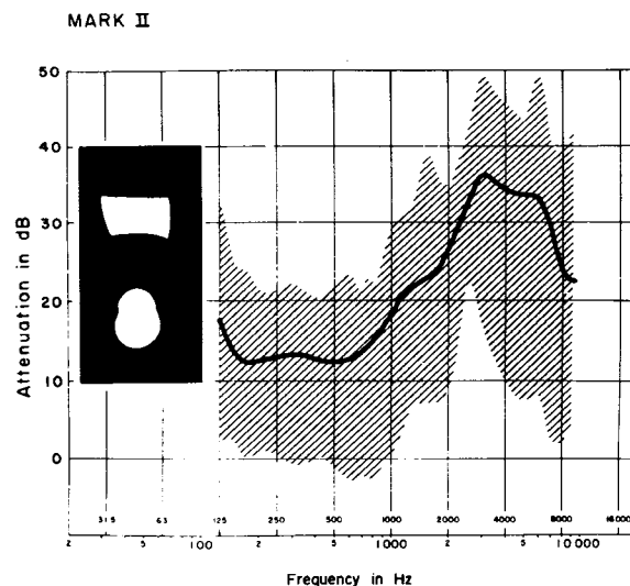
FIGURE 12. Measured attenuation provided by Mark II. The line represents the mean attenuation; the shaded area represents the range.
