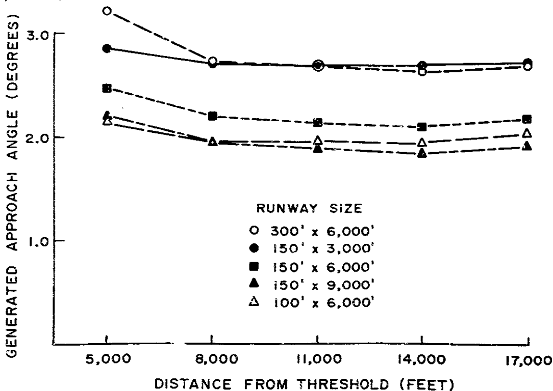
Figure 5. The effect on generated approach angles of runway size and distance from runway threshold.
