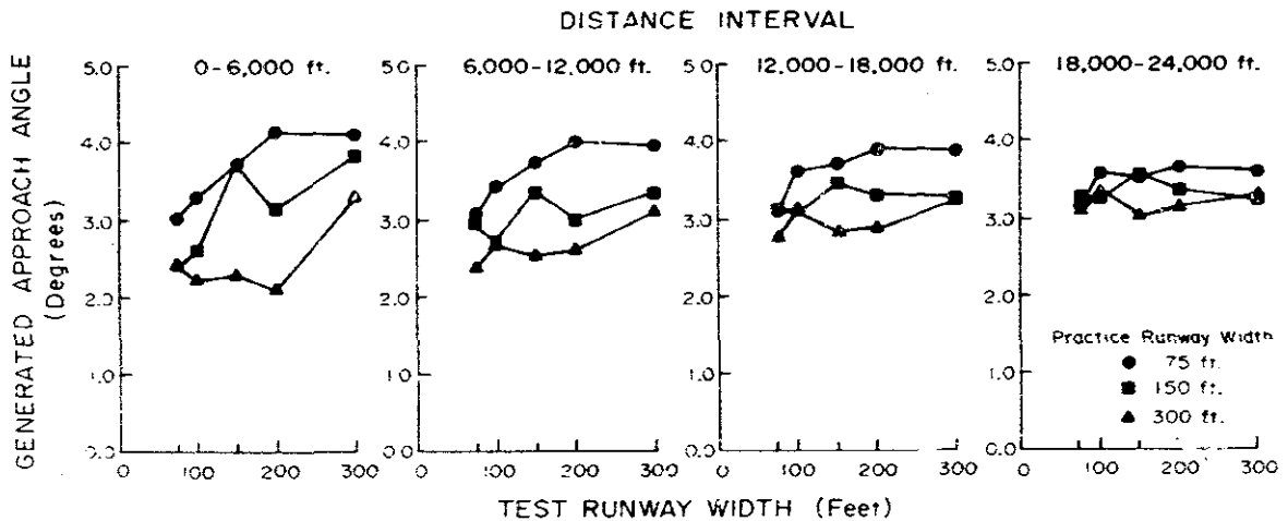
Figure 2. The effect of practice and test runway width in each of the four 1-nmi segments of approaches from 24,000 ft to threshold.
