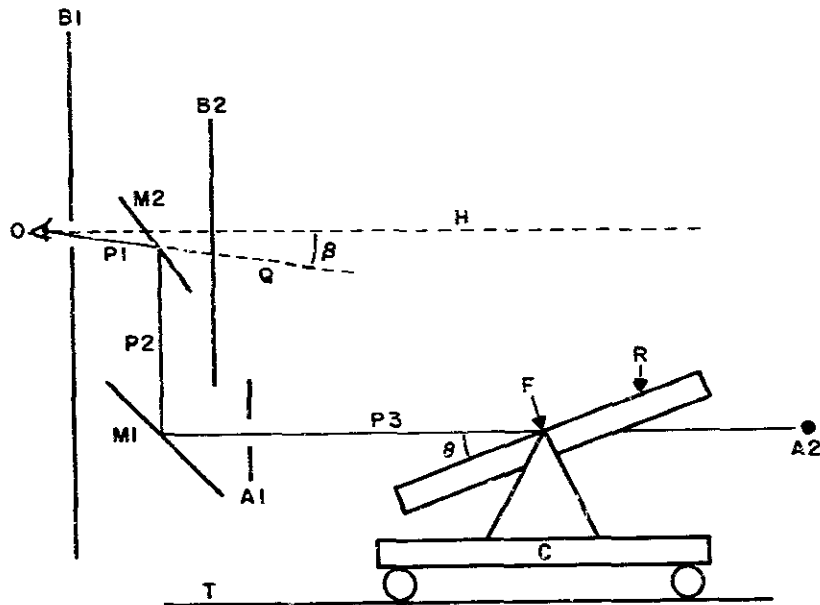
Figure 4. Schematic of apparatus (A1 and A2, removable targets for aligning optical system; B1 and B2, baffles; C, cart; F, rotation axis; H, horizontal line-of-sight; M1 and M2, mirrors; O, eye position; P1, P2, P3, segments of the optical axis; Q, apparent axis of radial motion; R, runway model; T, track; B, viewing angle; \theta , model slant.
