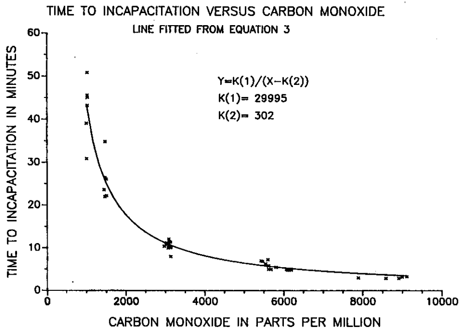
Figure 3. Scatter plot of time-to-incapacitation vs carbon monoxide concentration.
