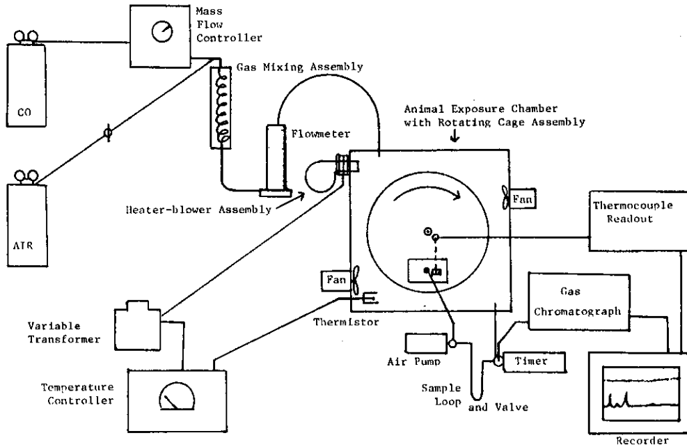
Figure 2. Animal Exposure System
