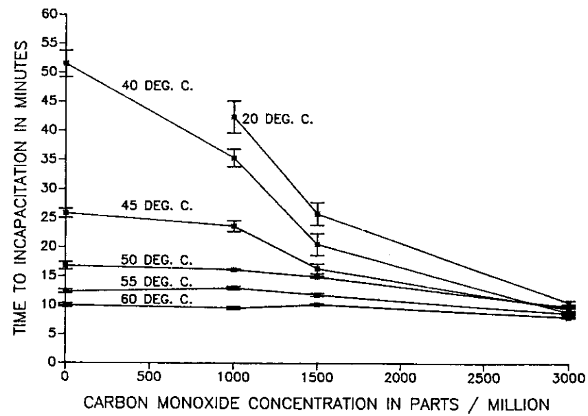
Figure 7. Variation in time-to-incapacitation with carbon monoxide concentration at 5 temperatures.
