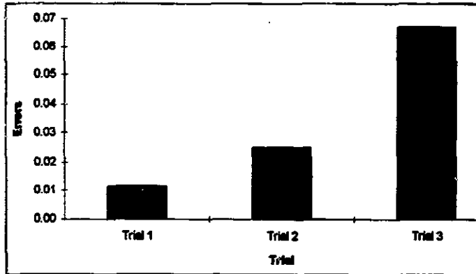
Figure 24. Communications Errors
