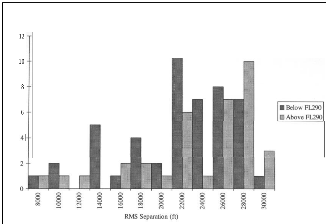
FIGURE 15. MINIMUM RMS SEPARATION FOR OEs
