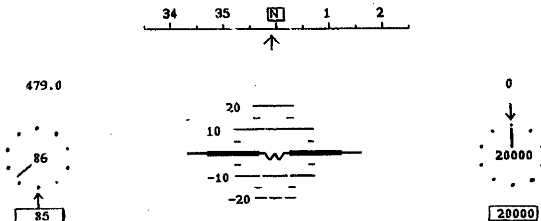
Figure 1. Symbology set: a heading scale, a pitch ladder with a horizon line, an airspeed indicator, an altimeter, a distance measuring equipment (DME) readout, and a digital vertical velocity display.
