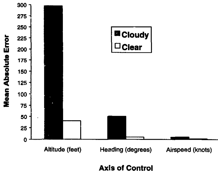
Figure 5. Tracking mean absolute error (MAE) by axis of control and weather condition
